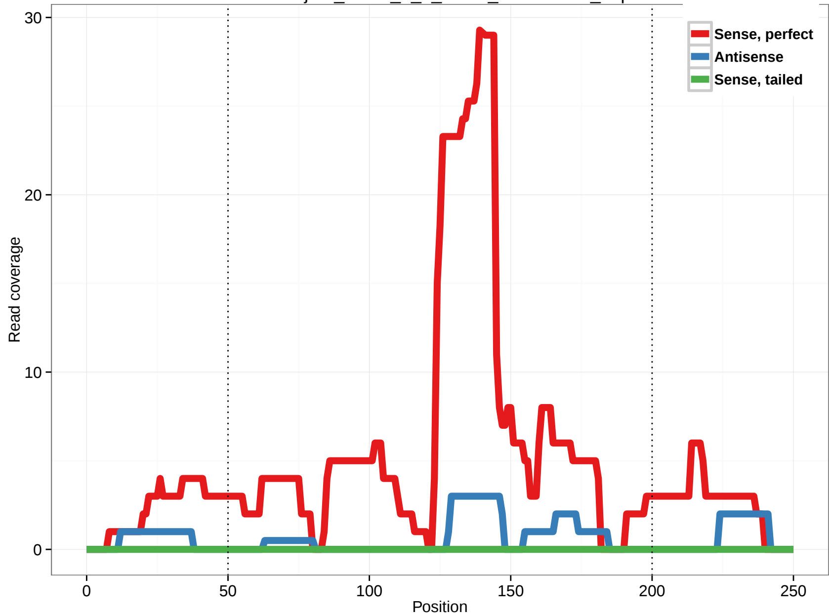
uc001tjd.2_intron_0_0_chr12_102514065_f.5p
