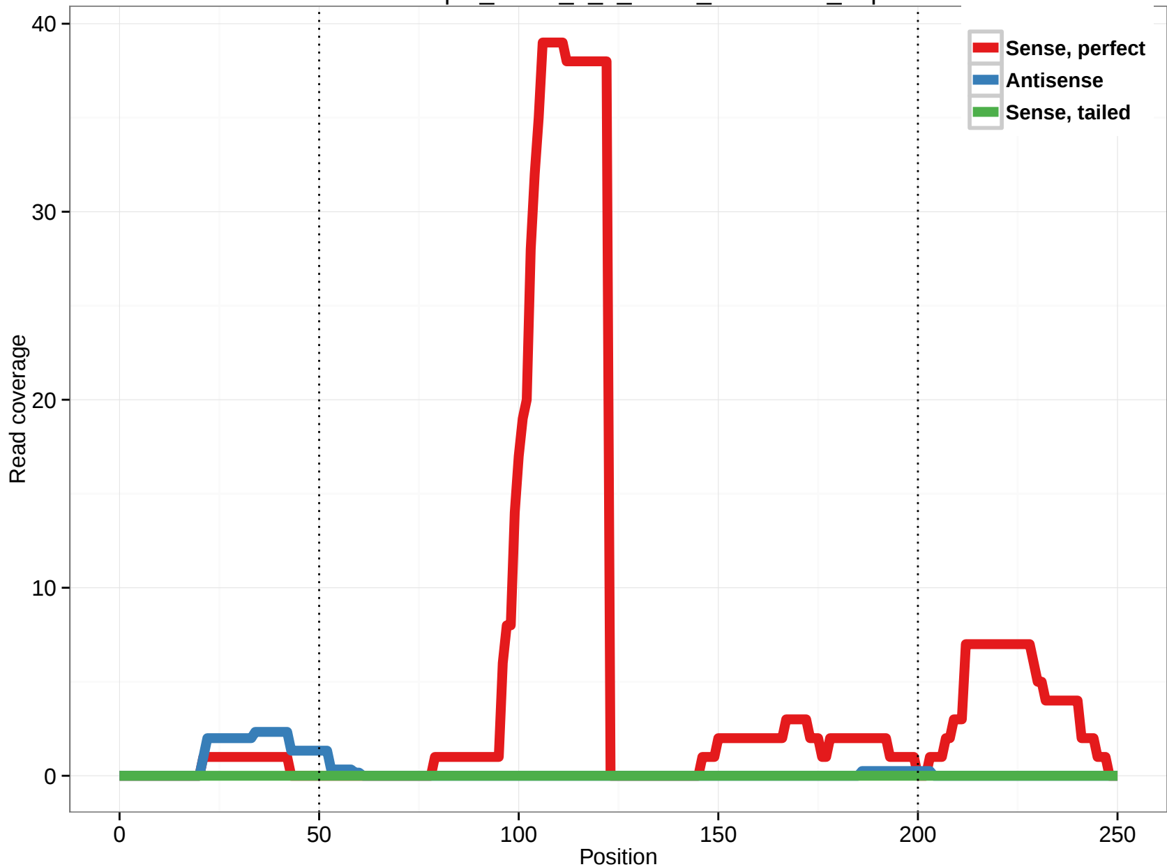
uc001tep.1_intron_9_0_chr12_96691500_r.3p
