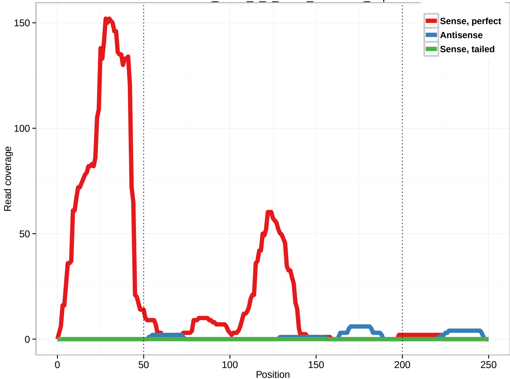
uc001tcs.2_intron_0_0_chr12_93861331_f.5p
