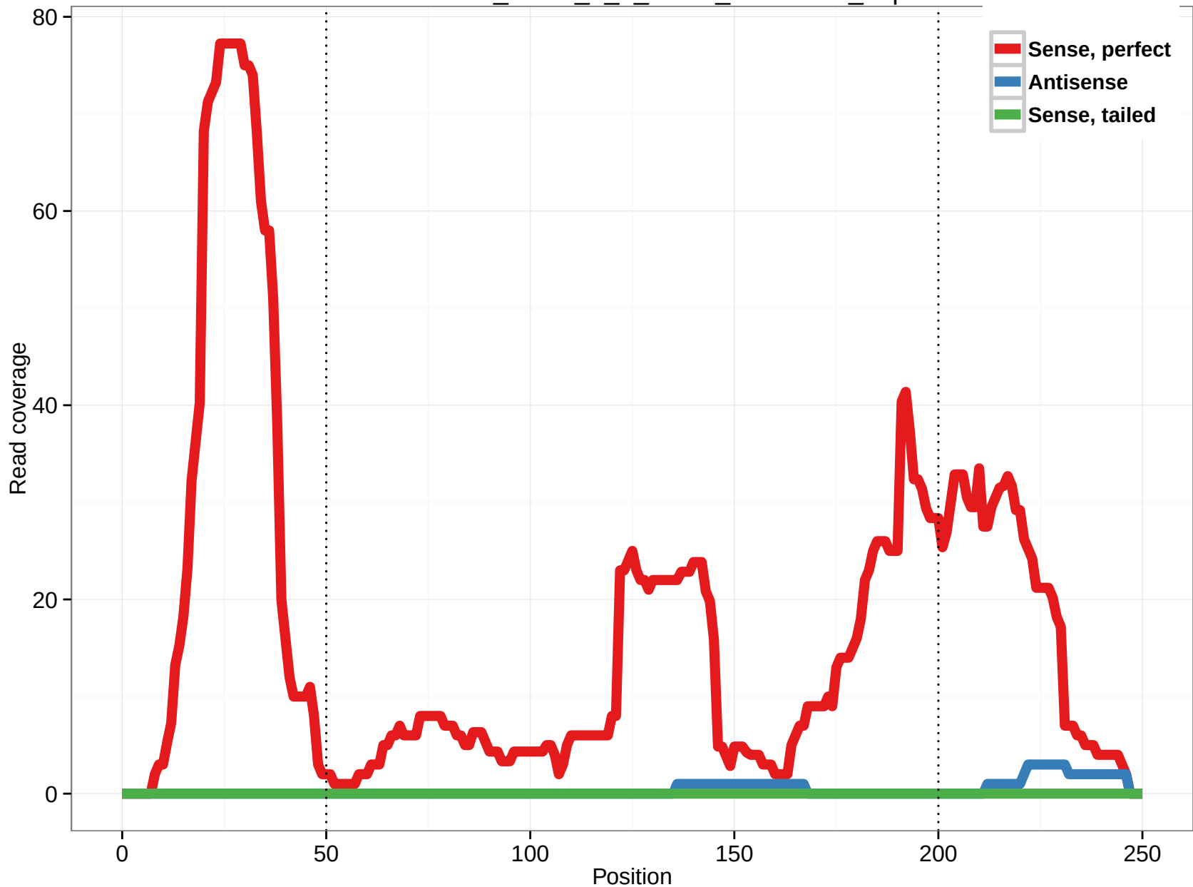
uc001suk.2_intron_3_0_chr12_69210667_f.3p
