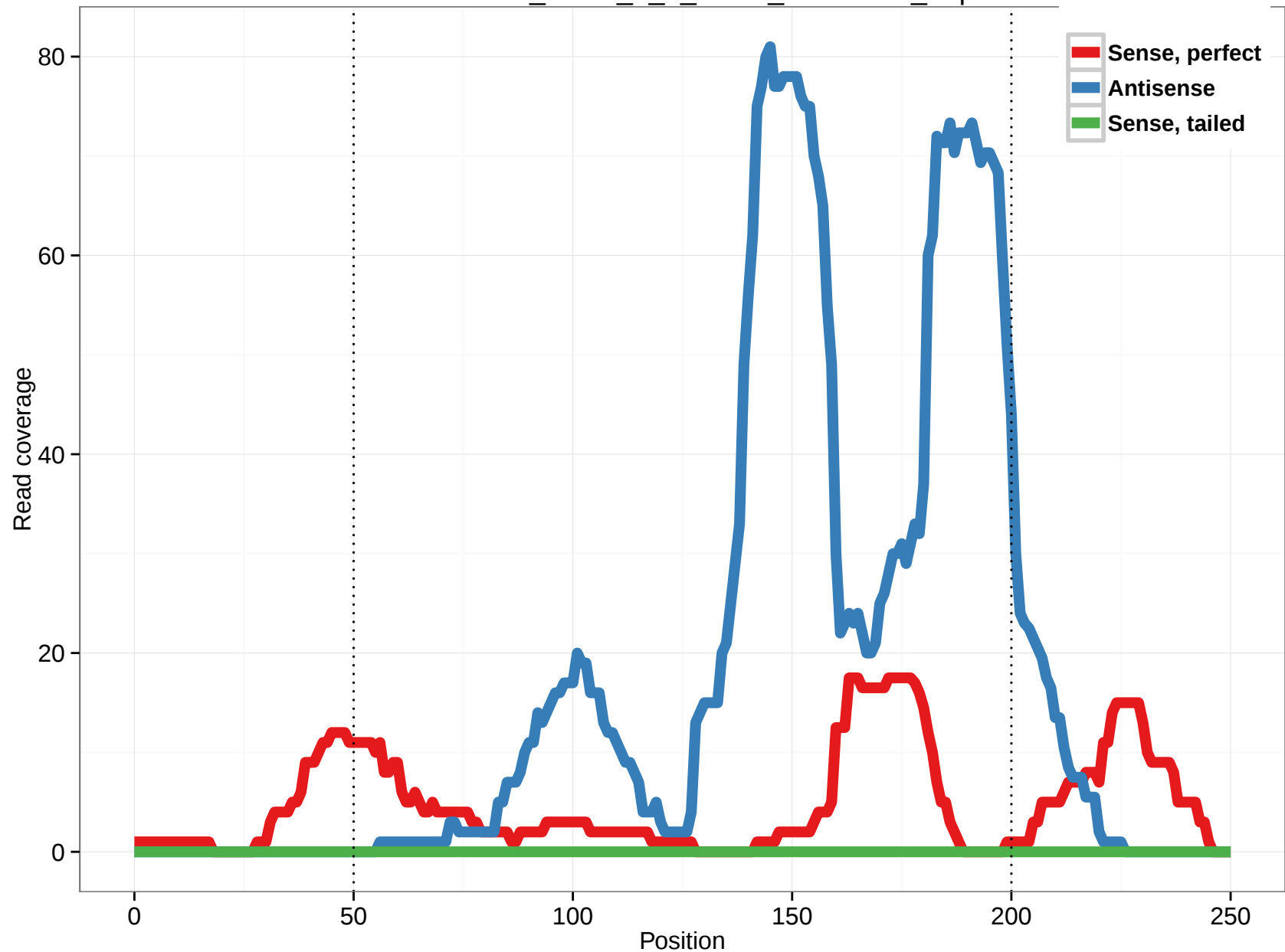
uc001ste.2_intron_6_0_chr12_66563134_r.3p
