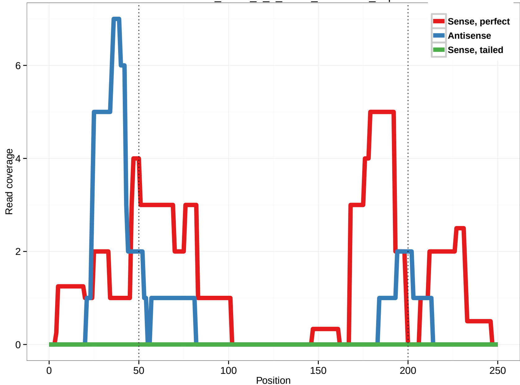
uc001smz.2_intron_0_0_chr12_57483138_f.5p
