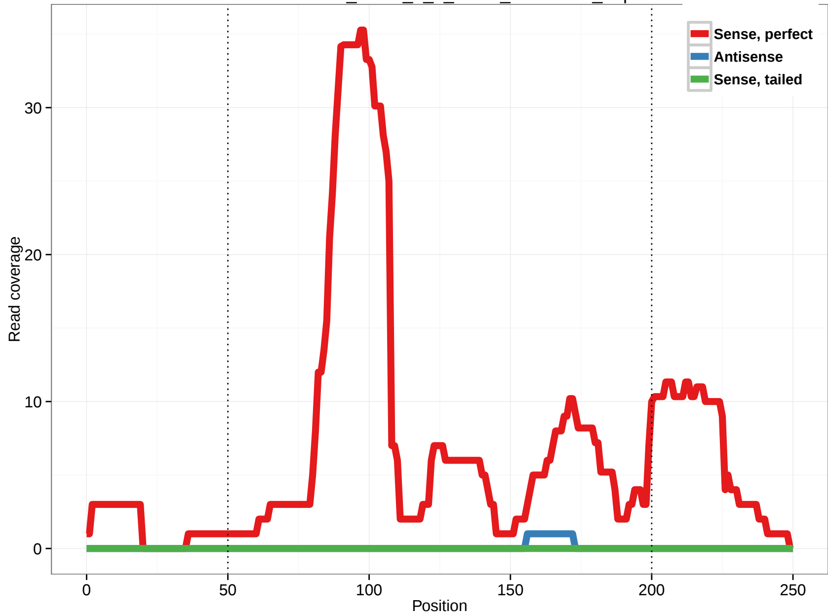
uc001sma.2_intron_6_0_chr12_57109991_r.5p
