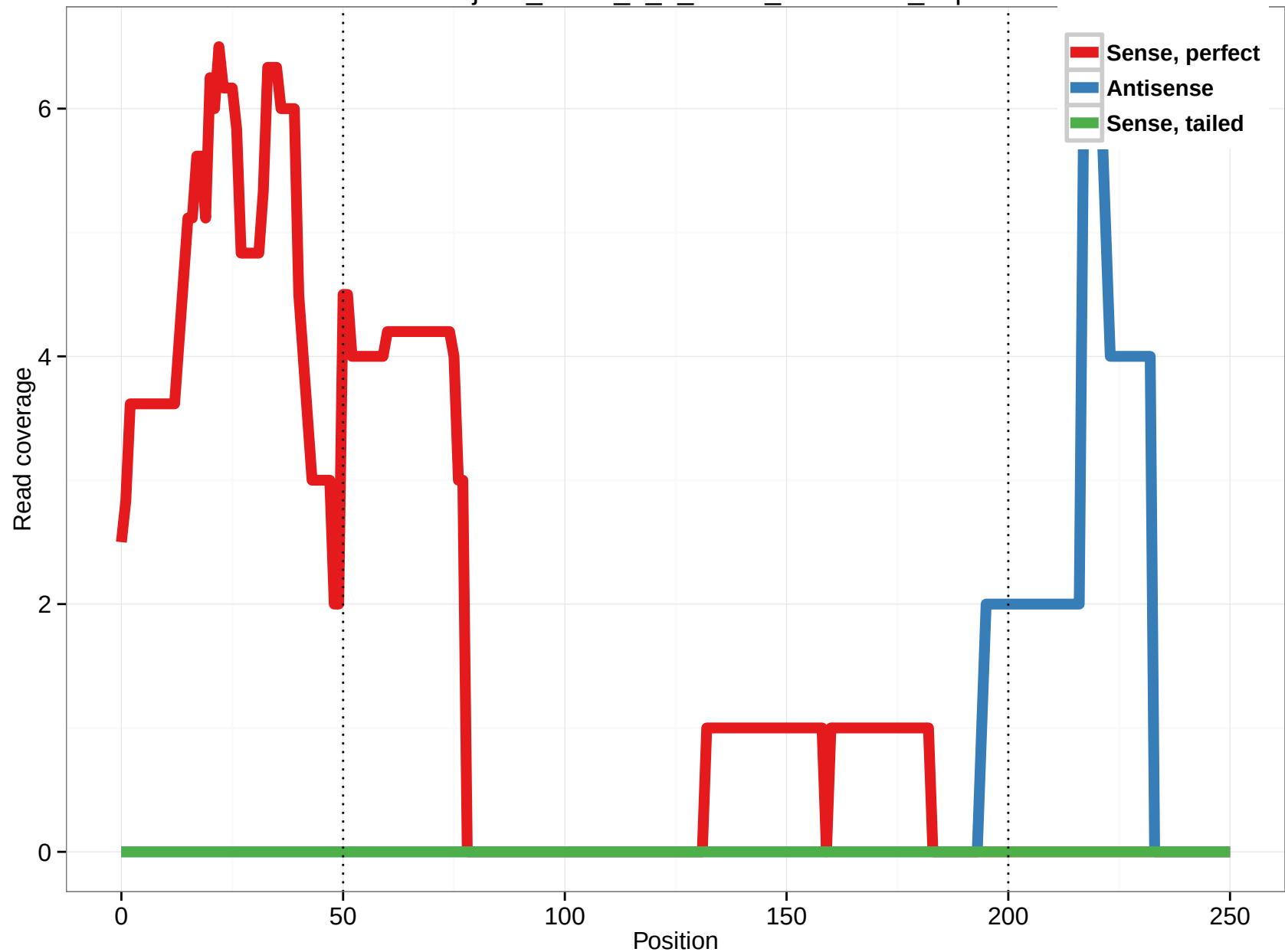
uc001sjm.2_intron_5_0_chr12_56503078_f.5p
