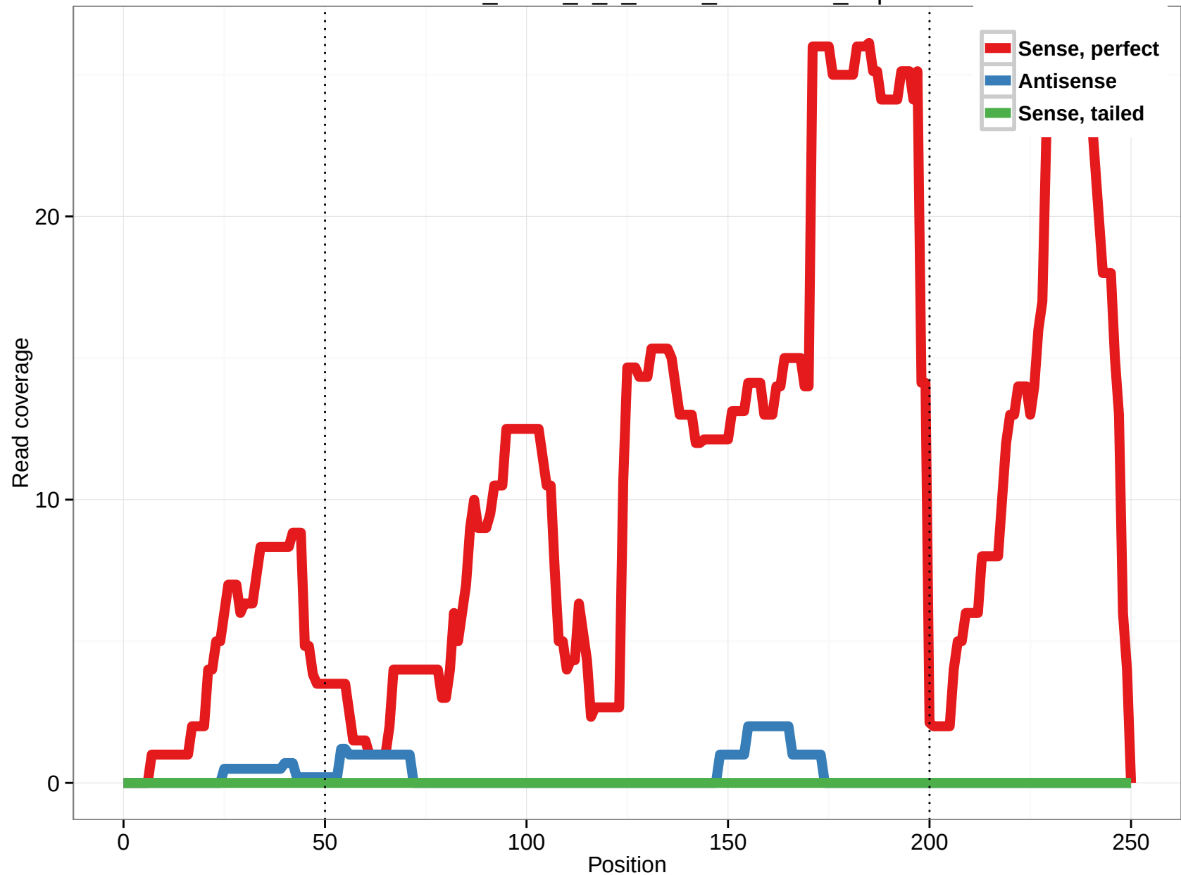
uc001sfl.2_intron_7_0_chr12_54677019_f.3p
