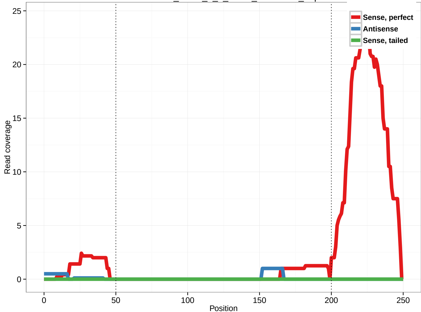
uc001sfh.3_intron_2_0_chr12_54646012_r.3p
