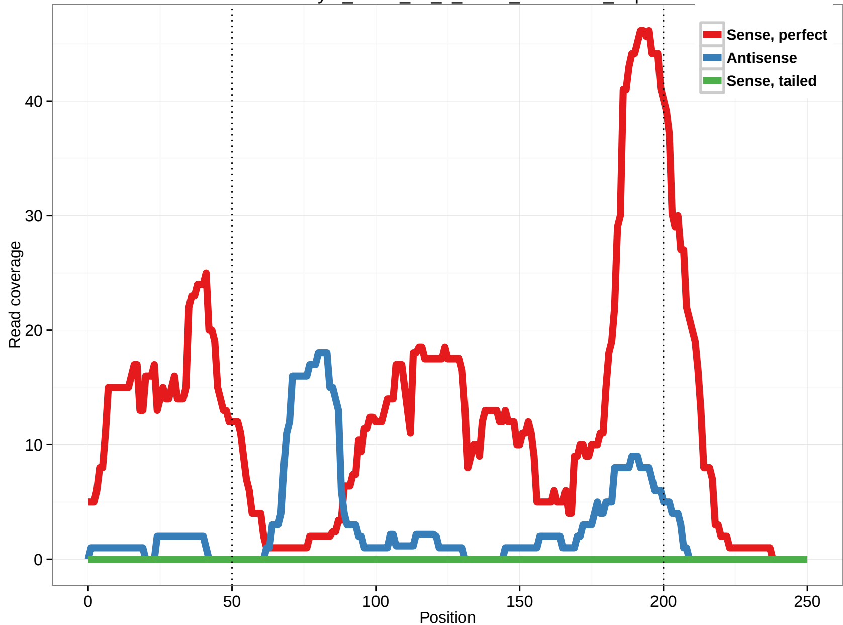
uc001roy.1_intron_10_0_chr12_46357972_r.5p
