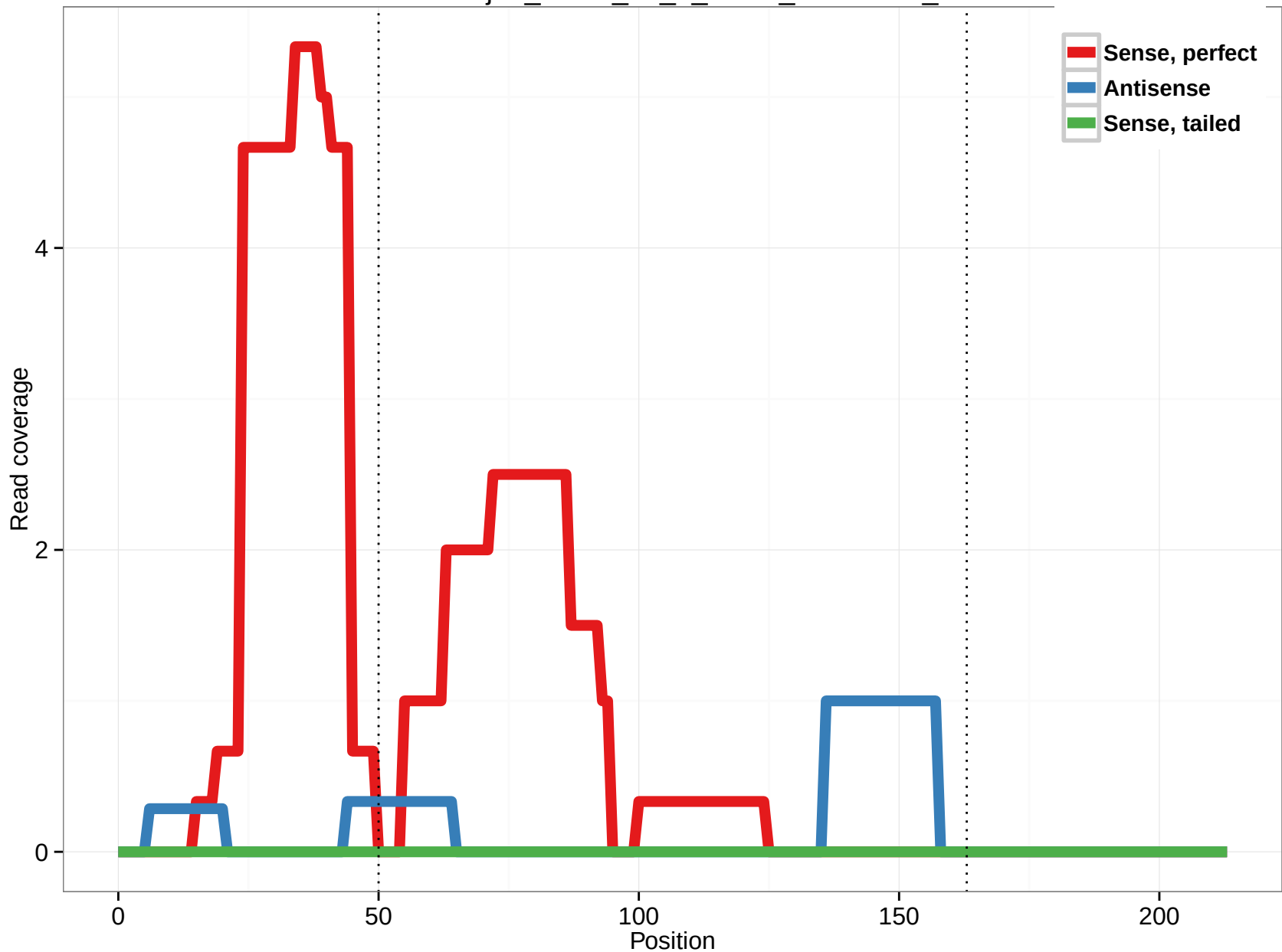
uc001rjr.1_intron_15_0_chr12_31249680_f
