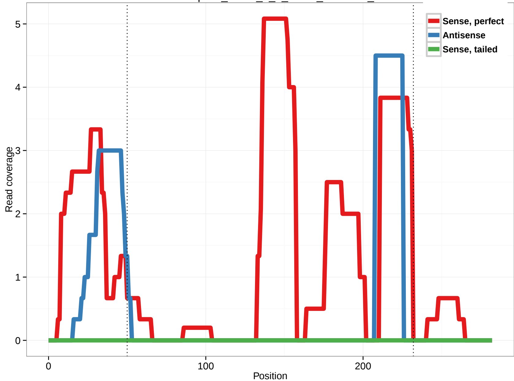
uc001qvx.3_intron_1_0_chr12_9571526_r
