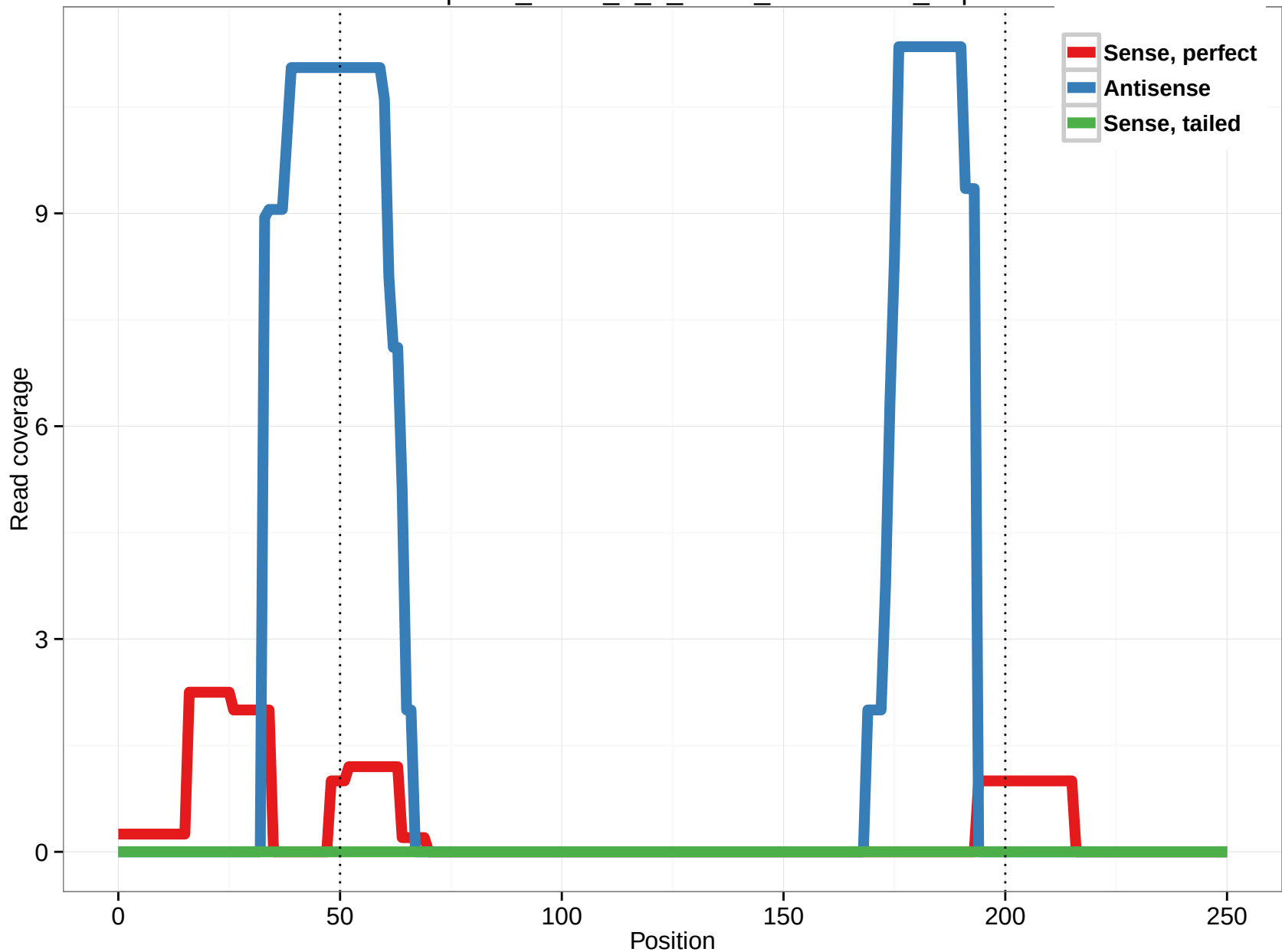
uc001phc.2_intron_3_0_chr11_102465489_r.3p
