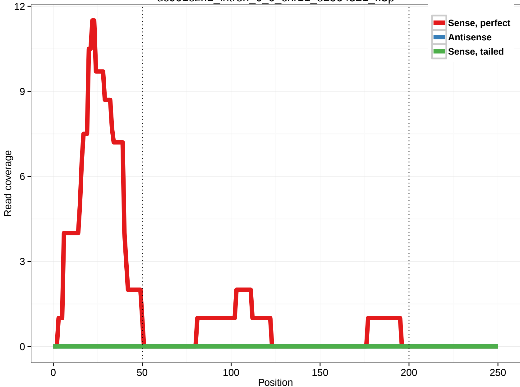
uc001ozr.2_intron_6_0_chr11_82564321_r.5p
