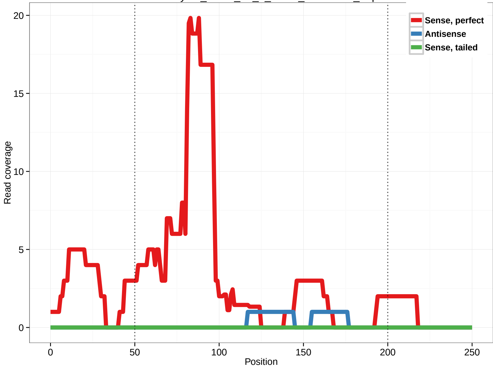
uc001oyz.1_intron_12_0_chr11_77838483_r.5p
