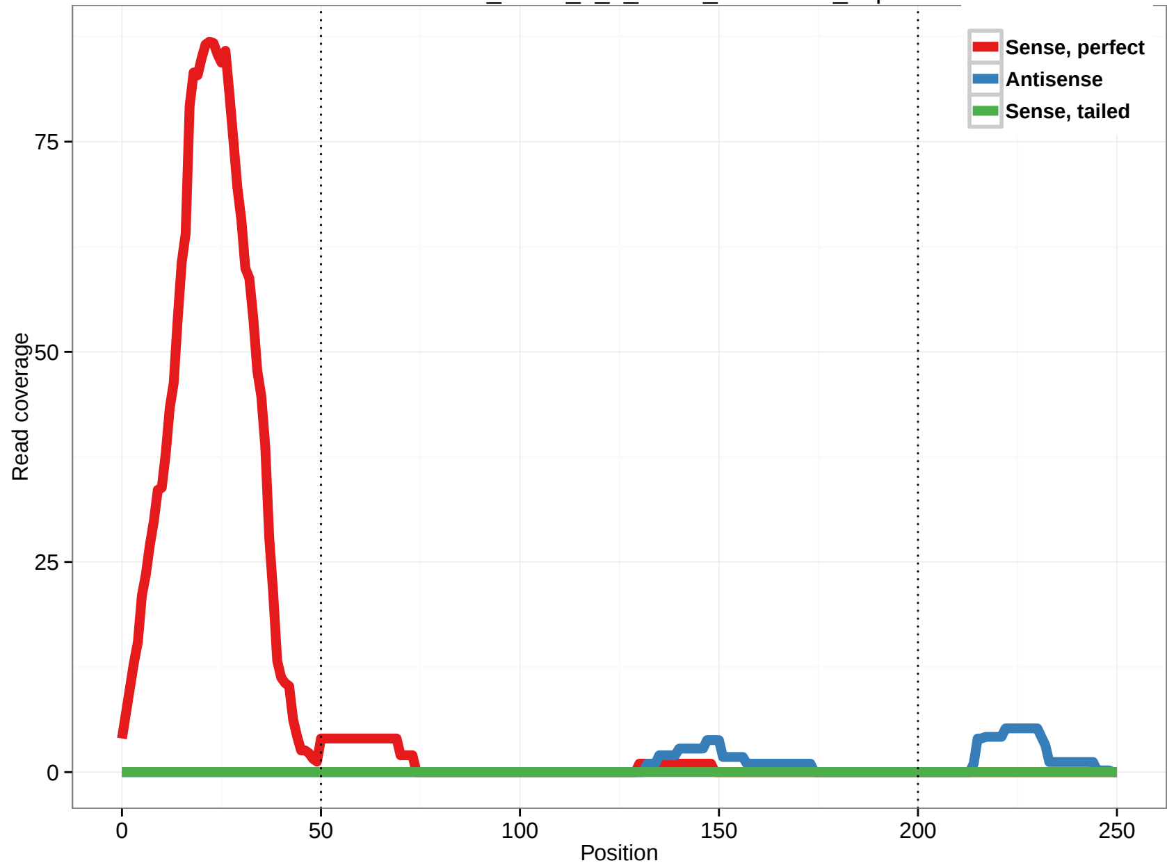
uc001owk.1_intron_0_0_chr11_75111869_f.5p
