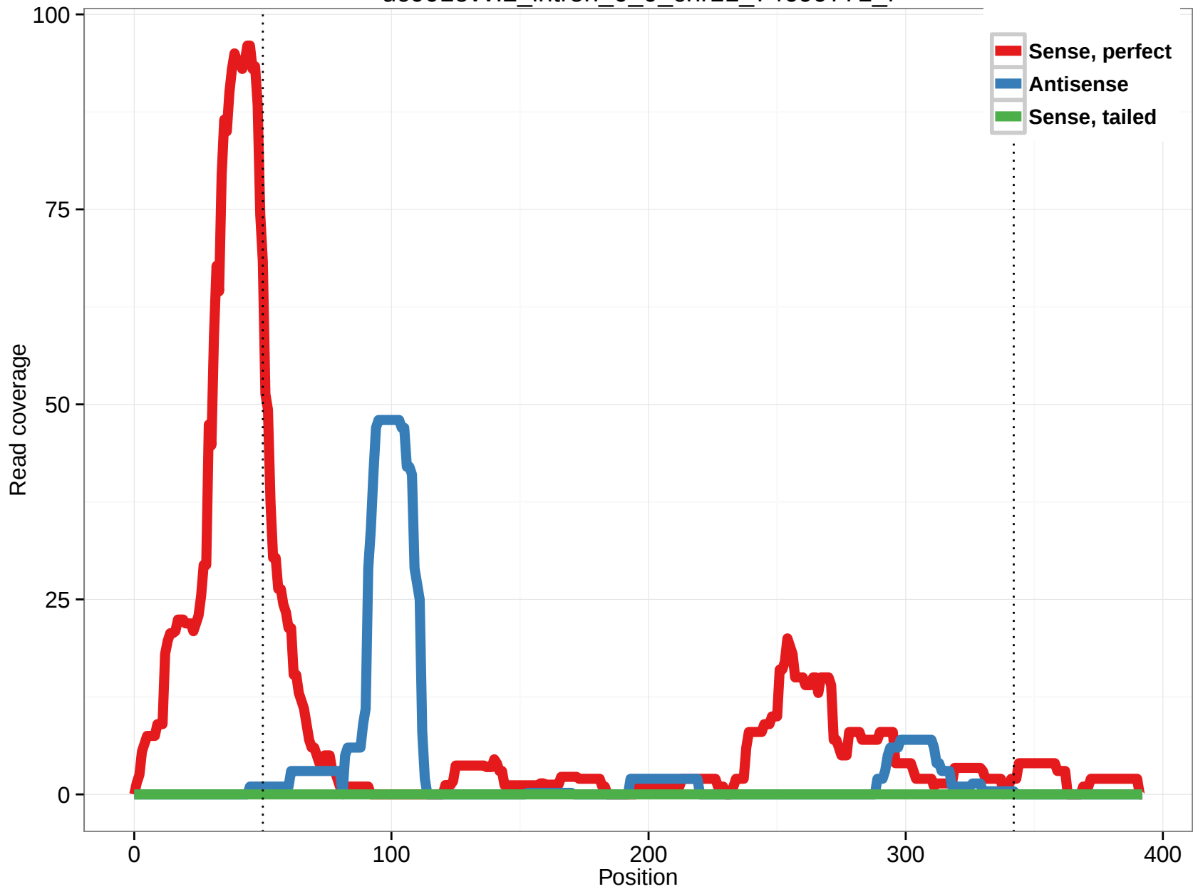
uc001ovv.2_intron_0_0_chr11_74699771_f
