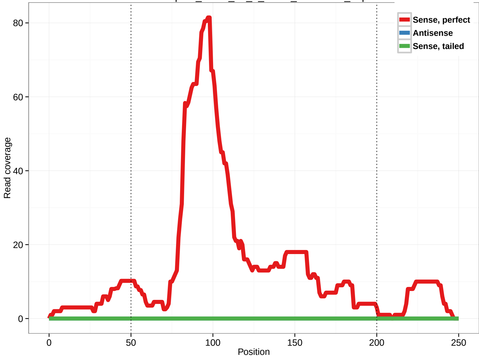
uc001opu.2_intron_17_0_chr11_70281851_f.3p
