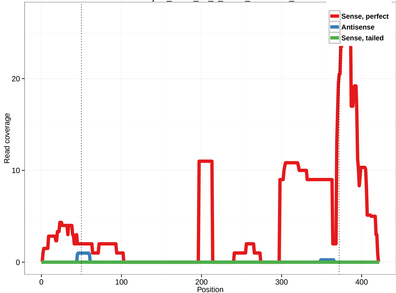
uc001ojd.2_intron_25_0_chr11_66475290_r
