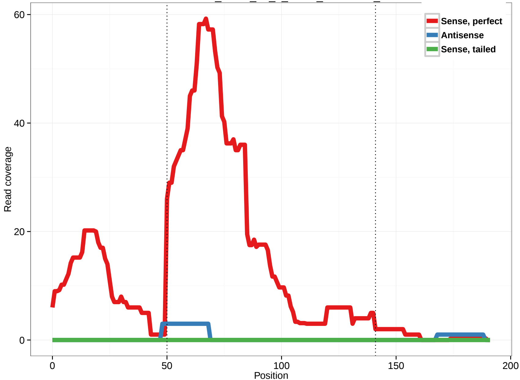
uc001ofv.3_intron_14_0_chr11_65633366_f
