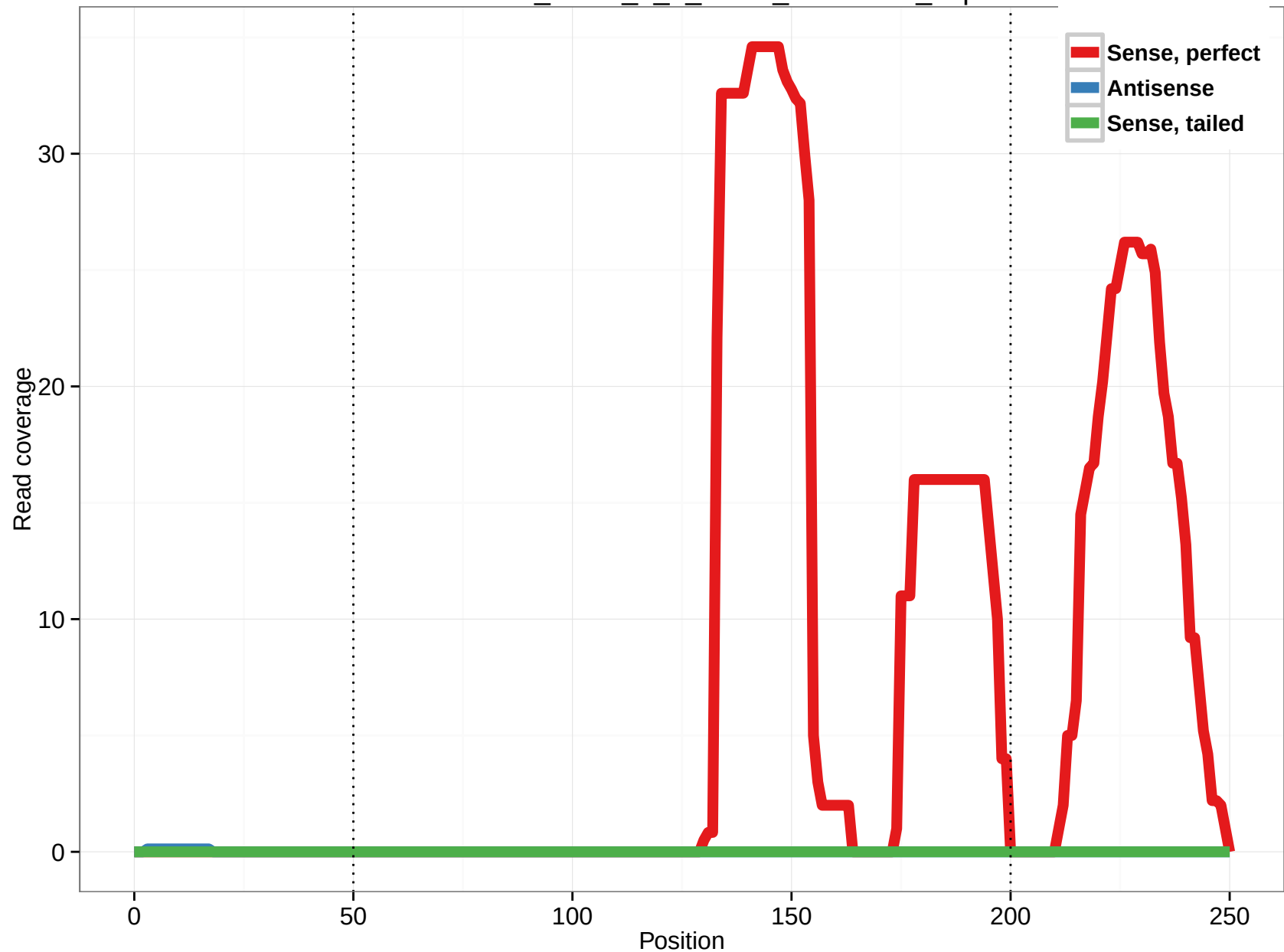
uc001oad.2_intron_3_0_chr11_64128065_f.3p
