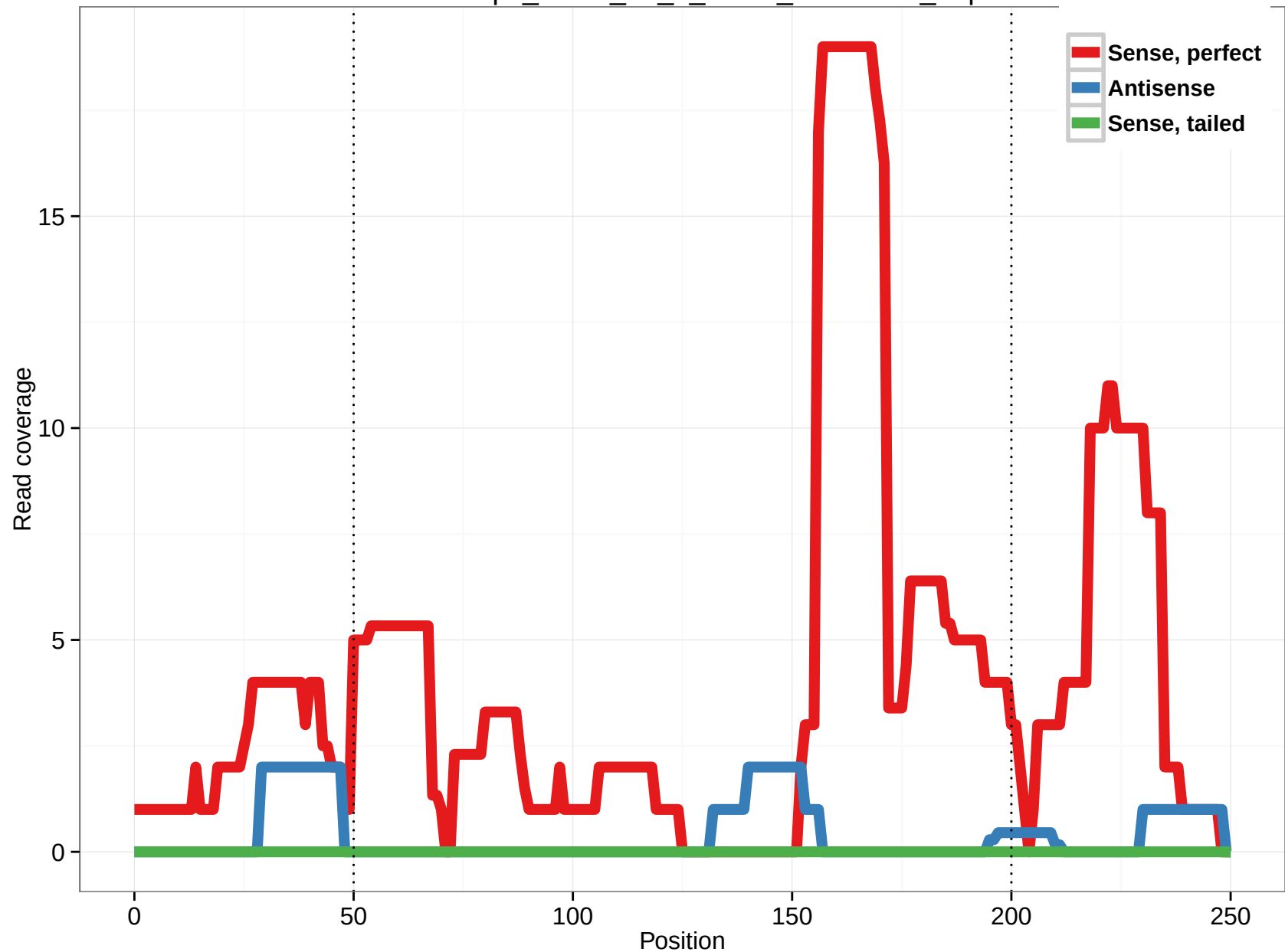
uc001ntq.1_intron_16_0_chr11_62368162_r.5p
