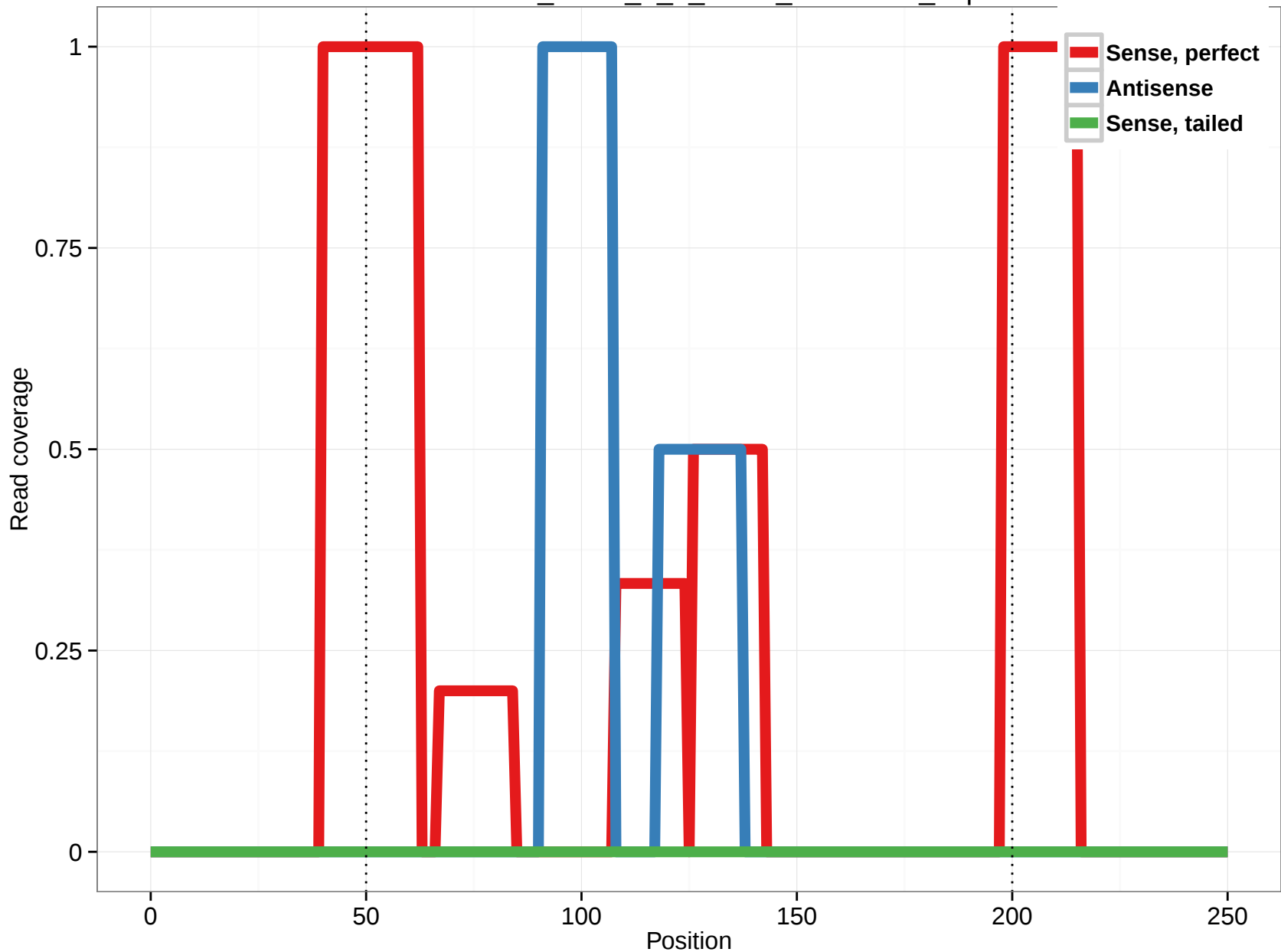
uc001nrz.1_intron_2_0_chr11_61396512_f.3p
