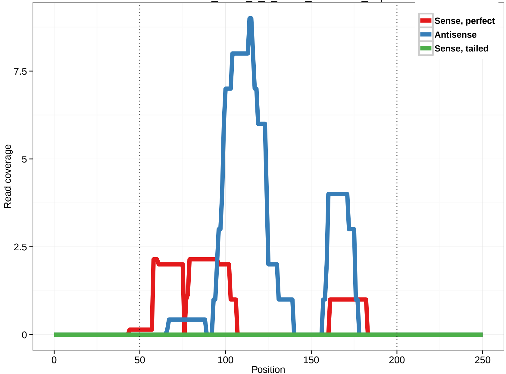
uc001muk.2_intron_1_0_chr11_33210397_f.3p
