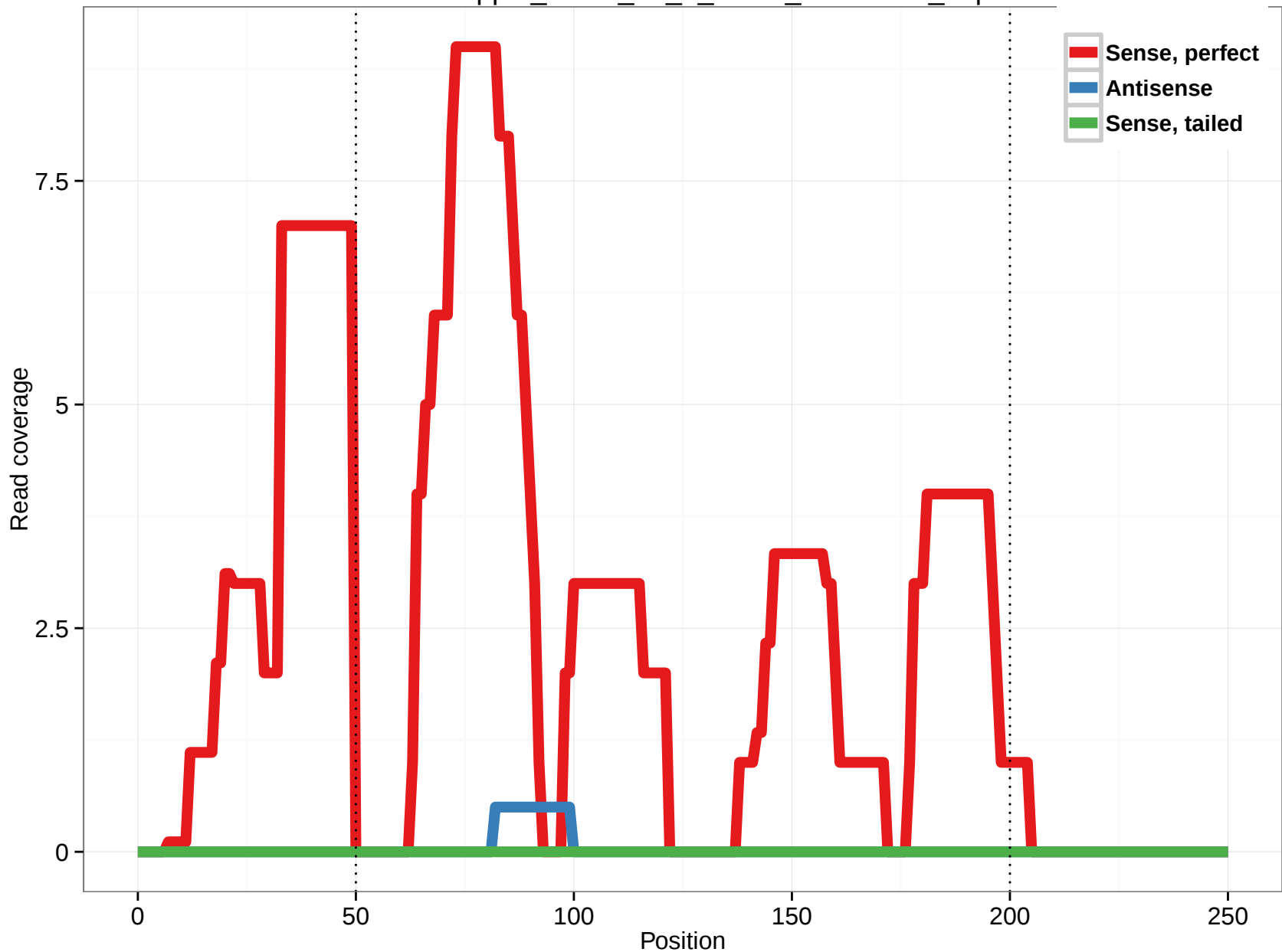
uc001mpp.2_intron_24_0_chr11_20101756_f.5p
