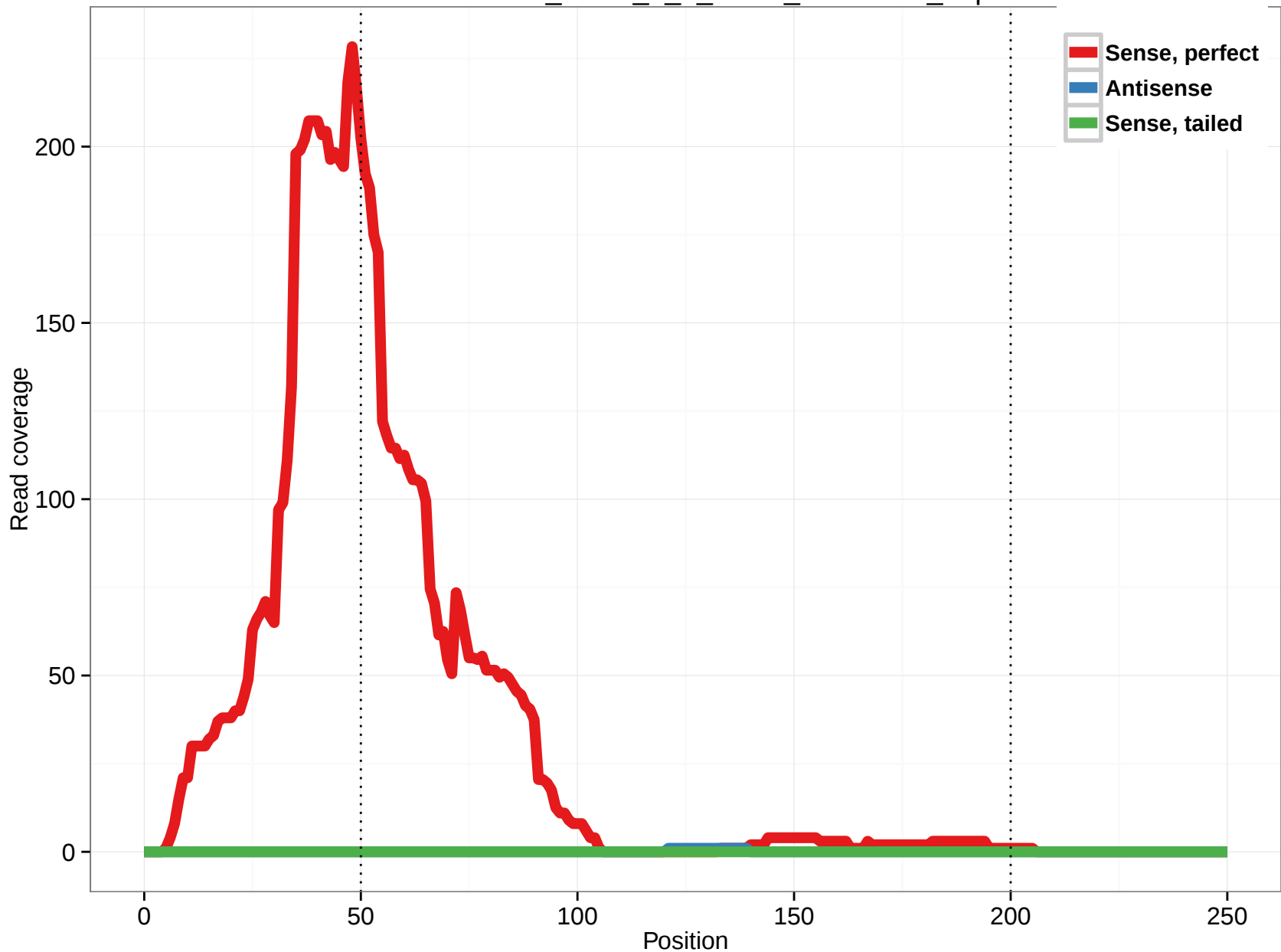
uc001mmh.1_intron_8_0_chr11_16758020_r.5p
