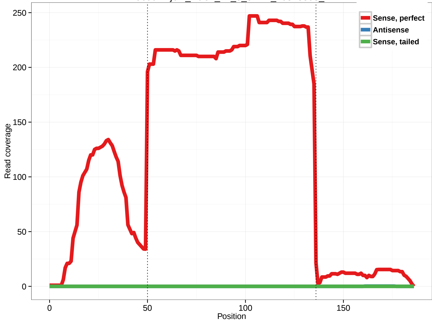
uc001mjb.2_intron_14_0_chr11_10825598_r
