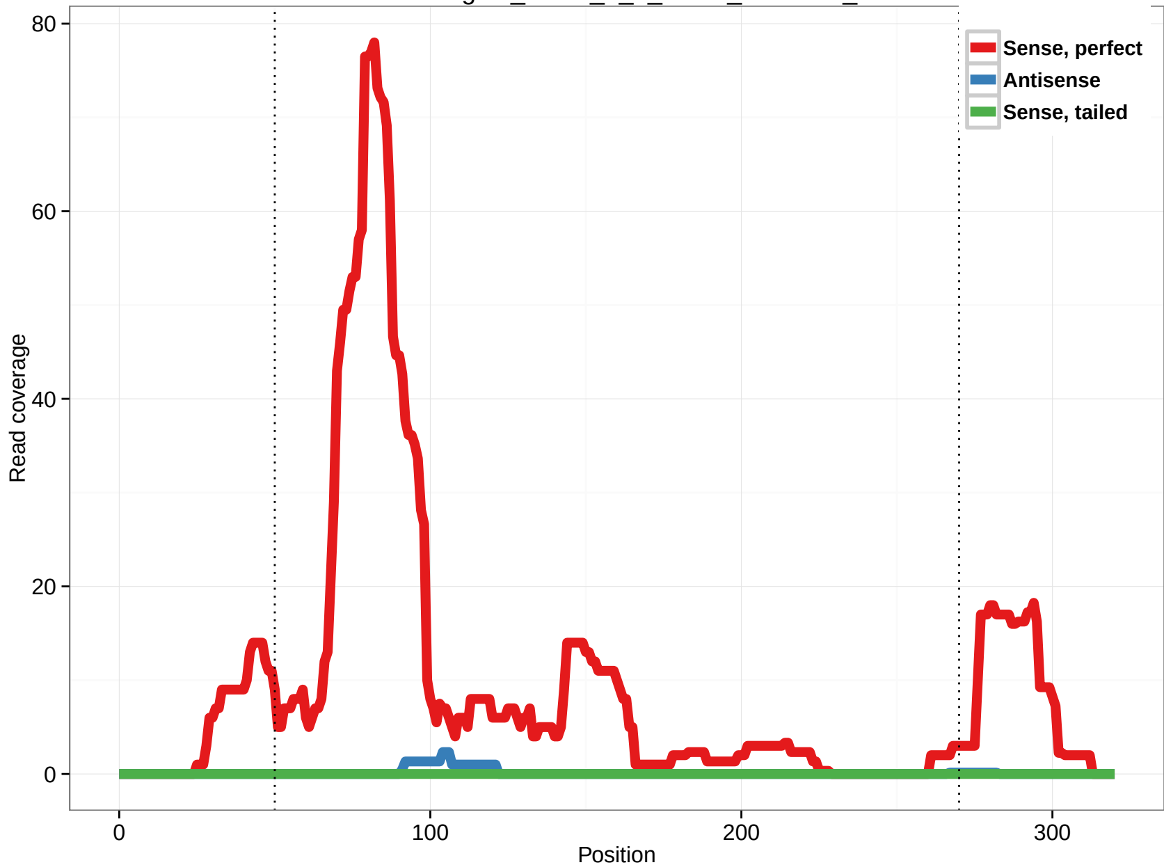
uc001mgx.2_intron_0_0_chr11_8932771_f
