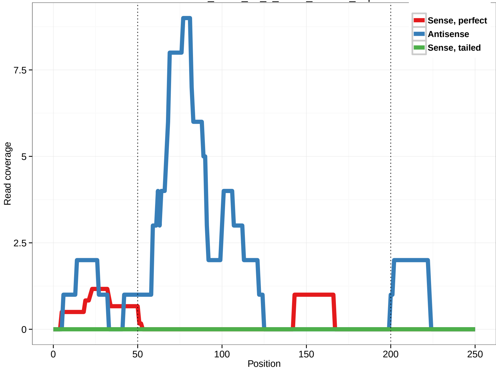
uc001lsn.2_intron_10_0_chr11_903112_r.5p
