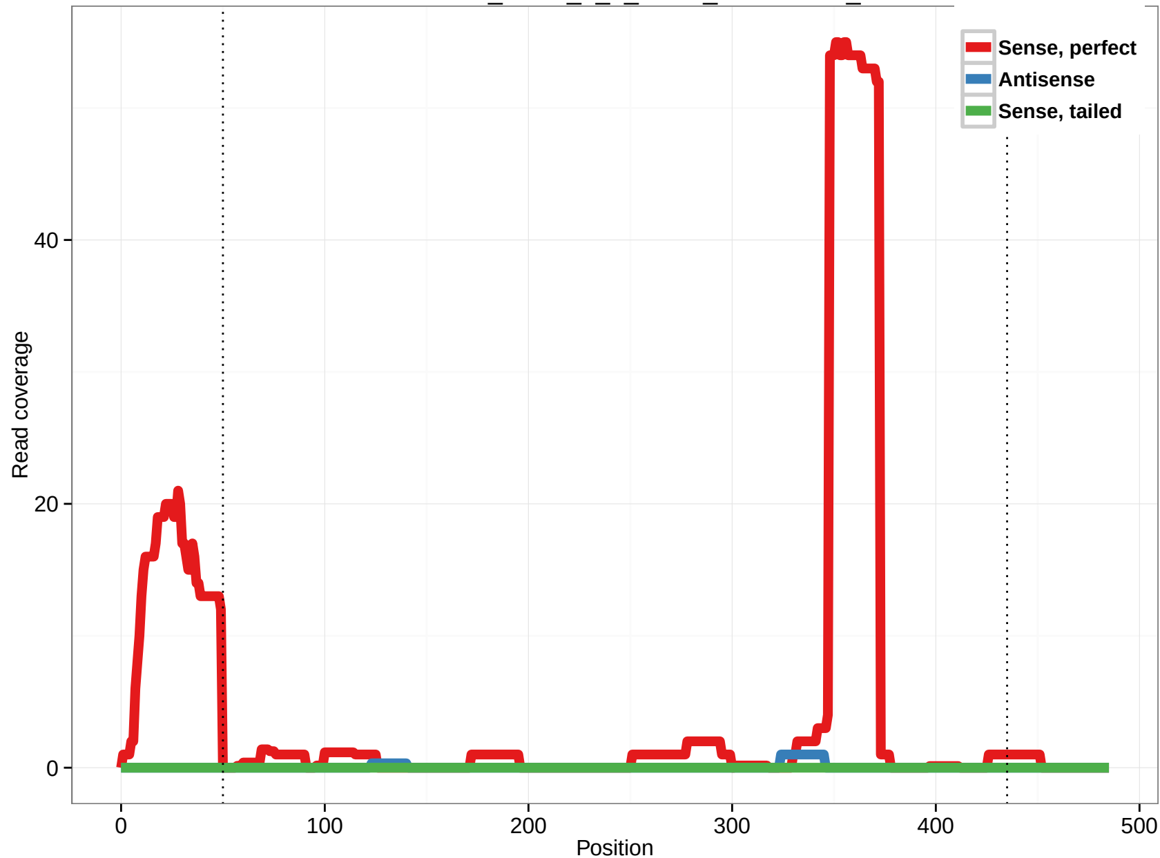
uc001Ind.2_intron_1_0_chr10_135209282_f
