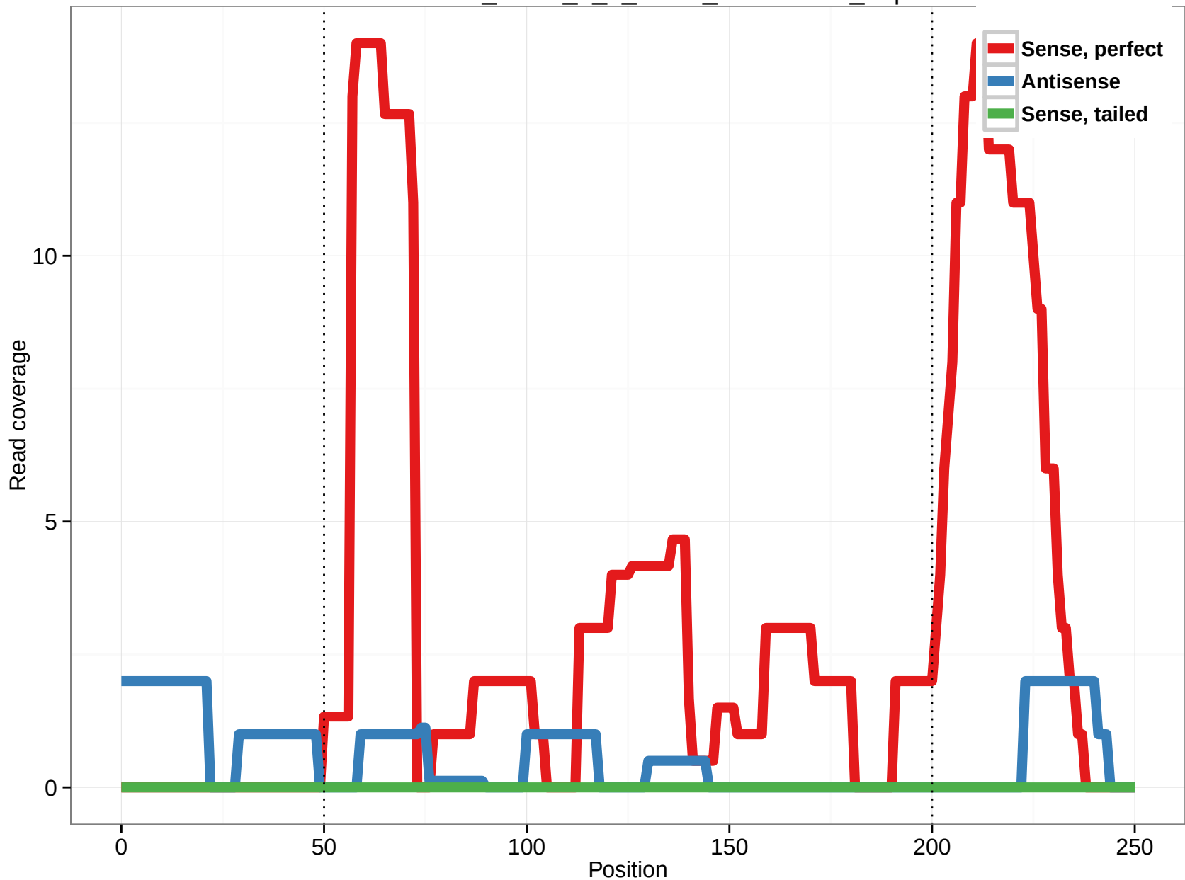
uc001lms.2_intron_4_0_chr10_135170760_r.3p
