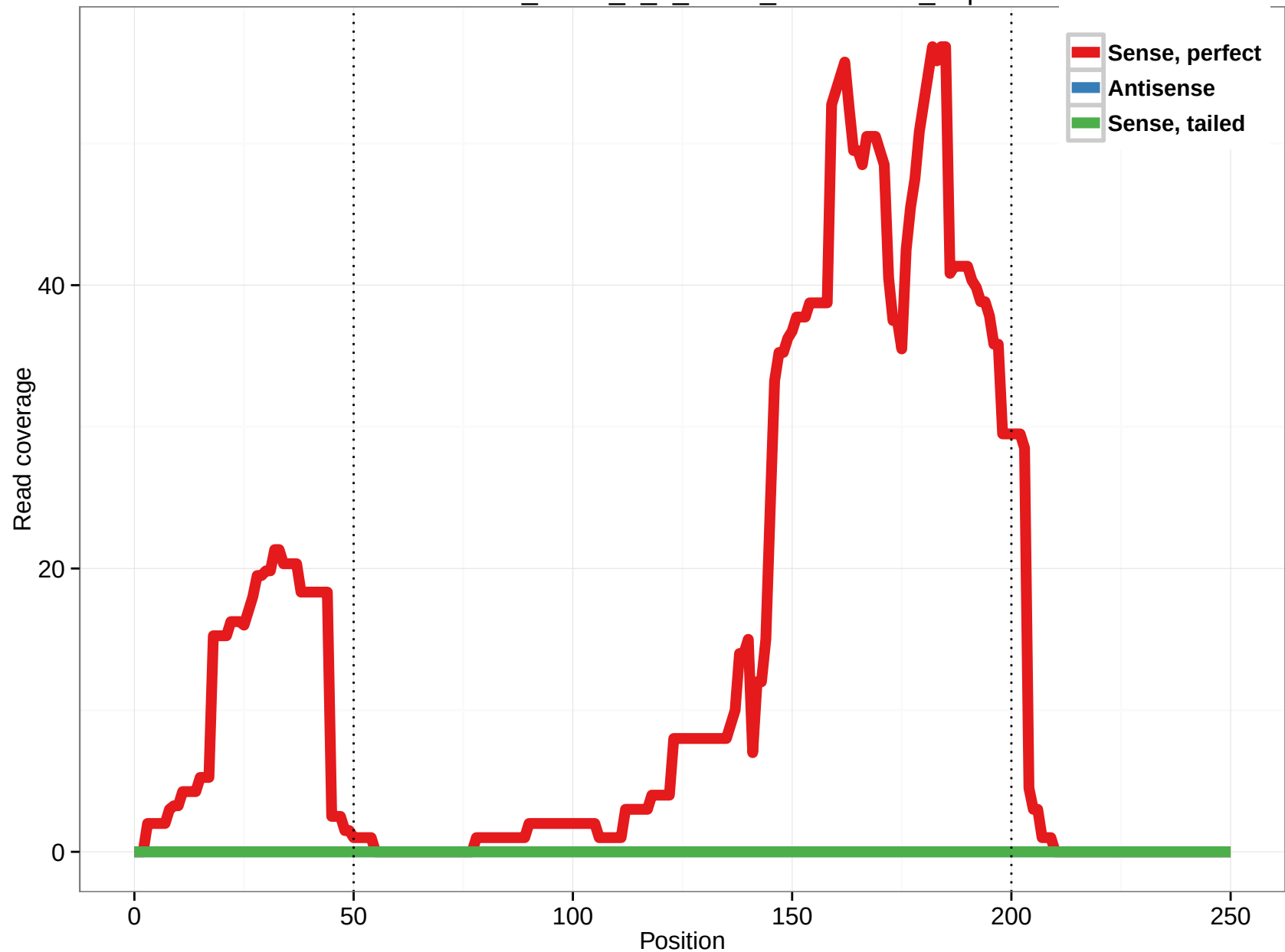
uc001leh.1_intron_6_0_chr10_121339523_r.5p
