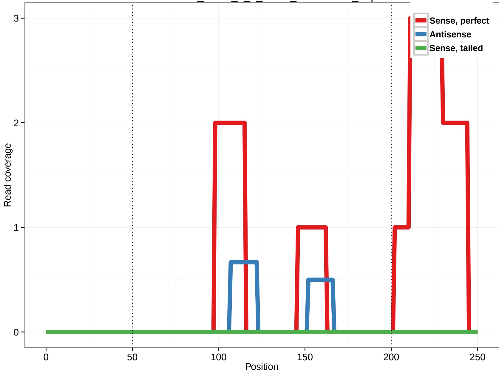
uc001lct.2_intron_1_0_chr10_118436014_r.3p
