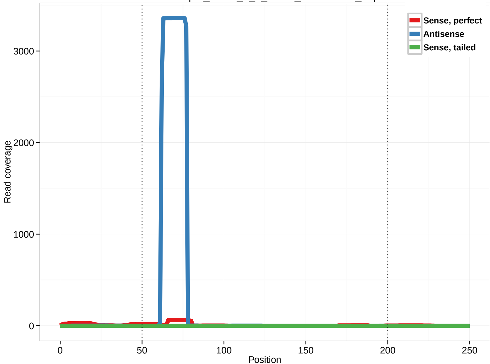
uc001lap.2_intron_0_0_chr10_115439738_f.5p
