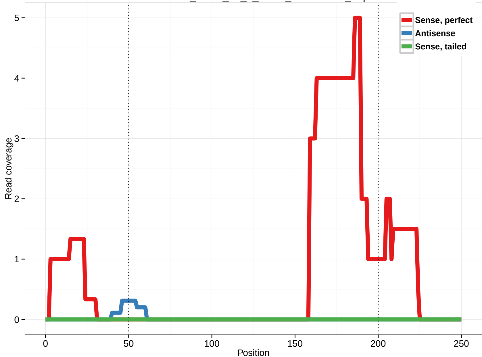
uc001kxr.2_intron_30_0_chr10_105810660_r.5p
