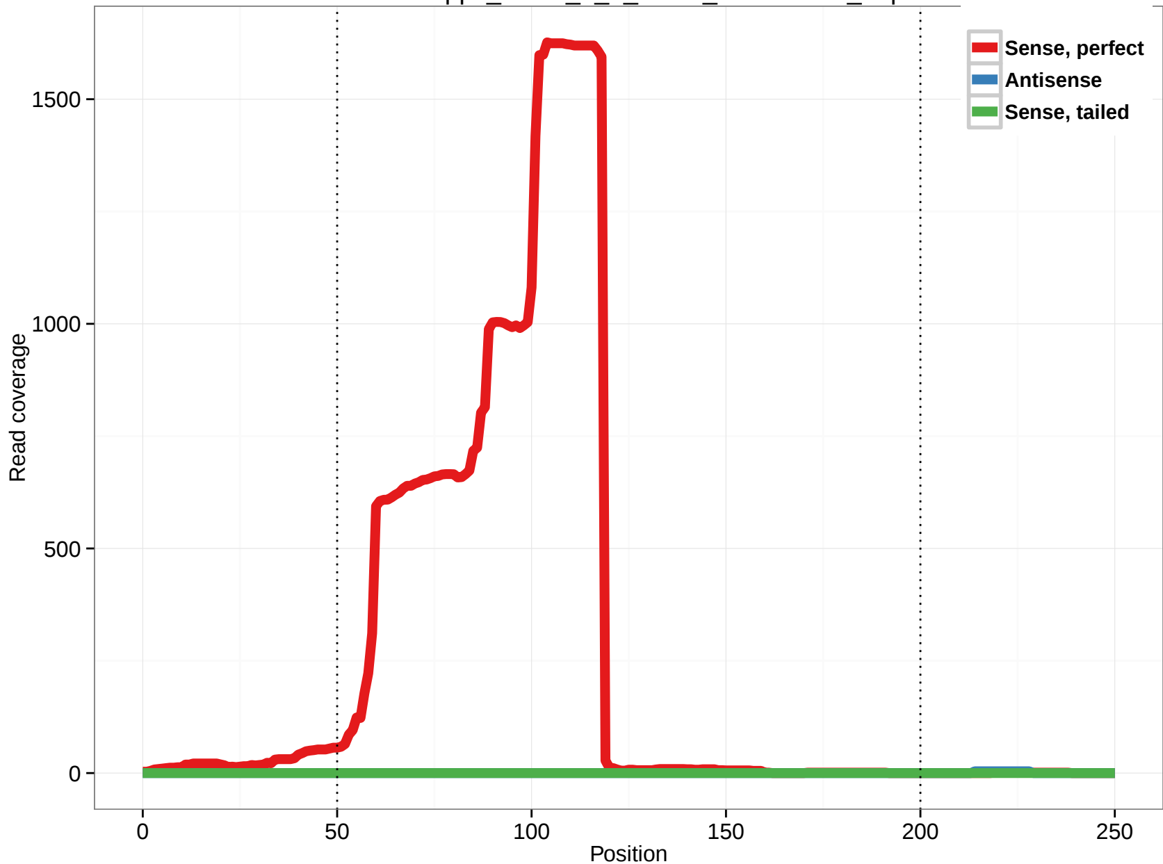
uc001kqq.1_intron_2_0_chr10_101996727_r.3p
