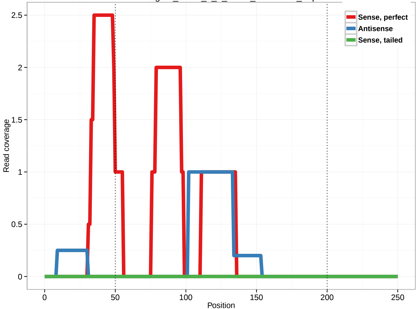
uc001kgd.2_intron_1_0_chr10_91053426_r.5p
