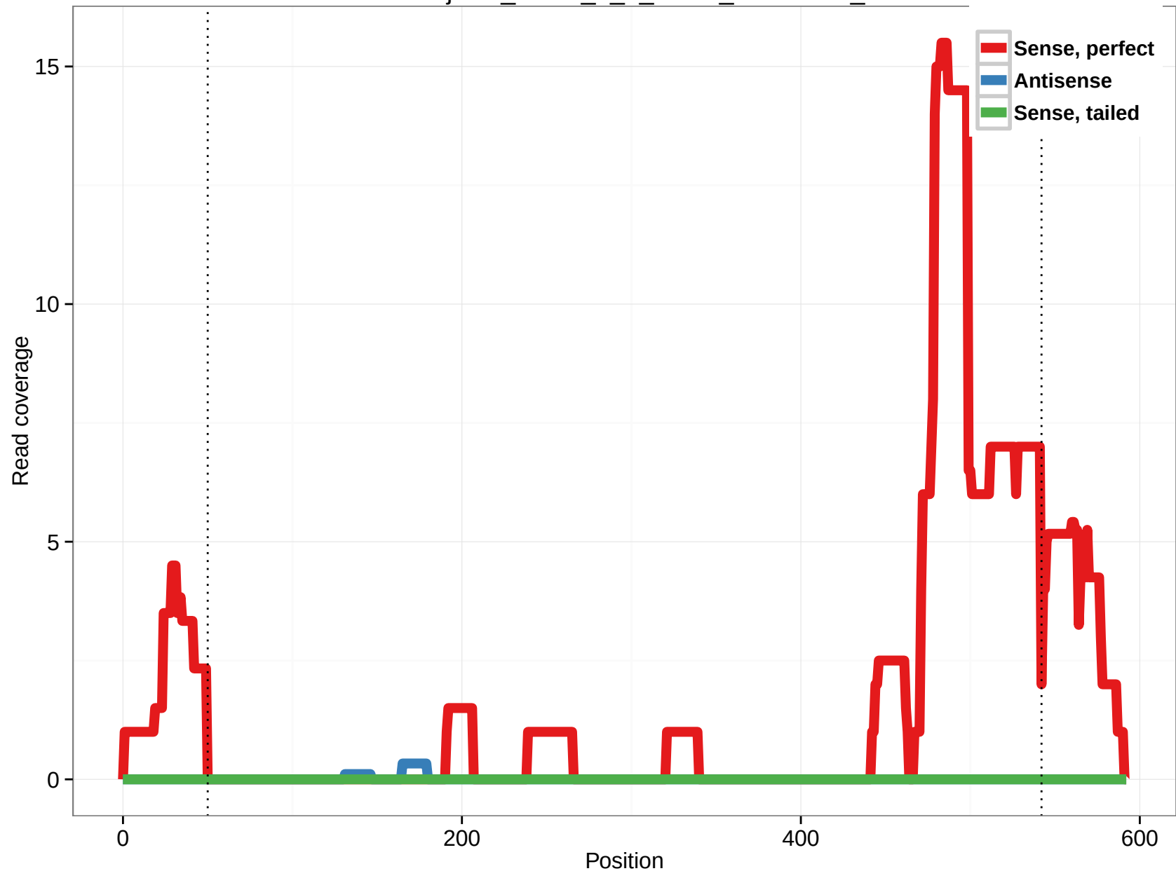
uc001jso.1_intron_3_0_chr10_73826879_r
