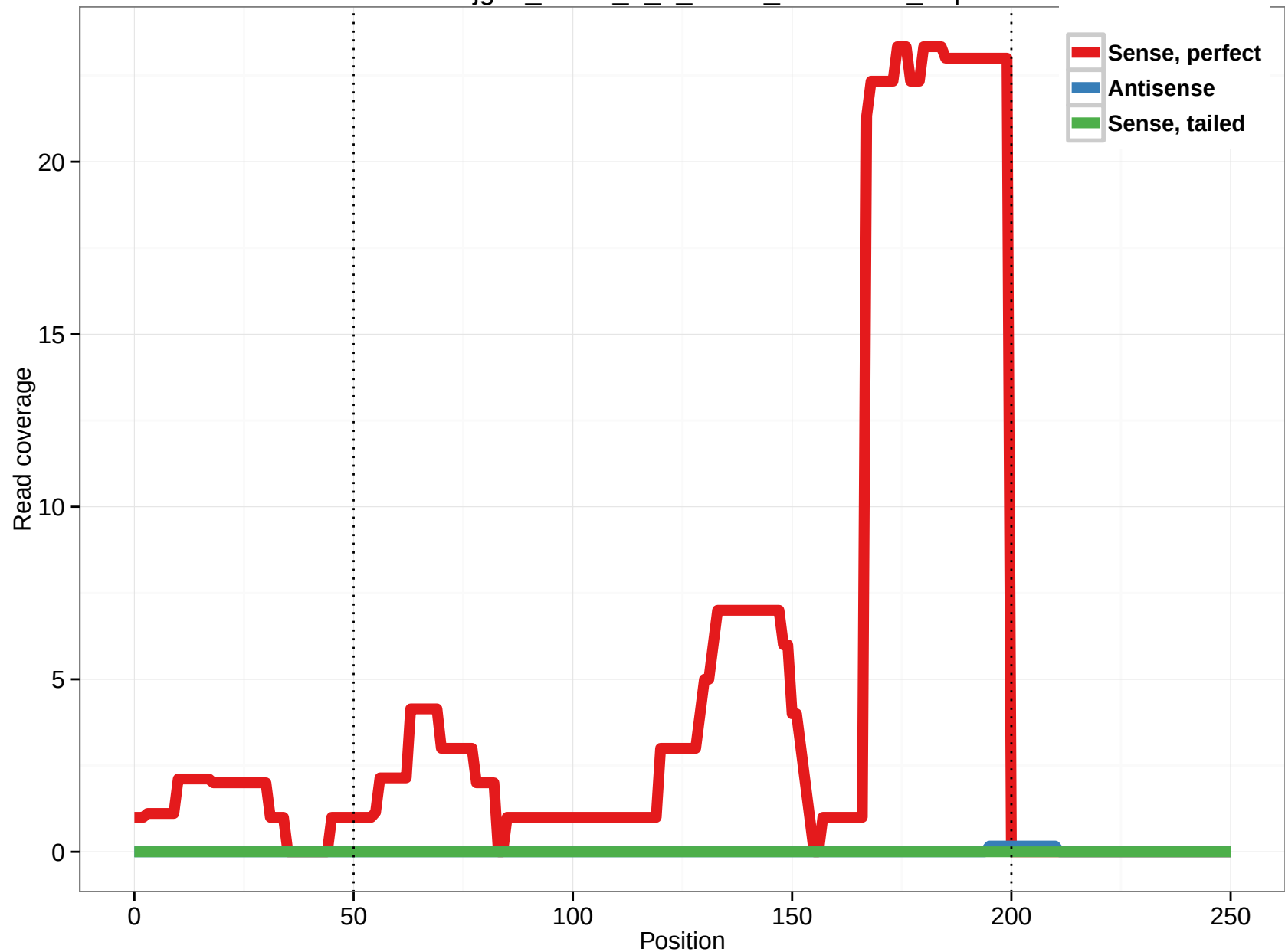
uc001jgl.2_intron_0_0_chr10_49514865_f.3p
