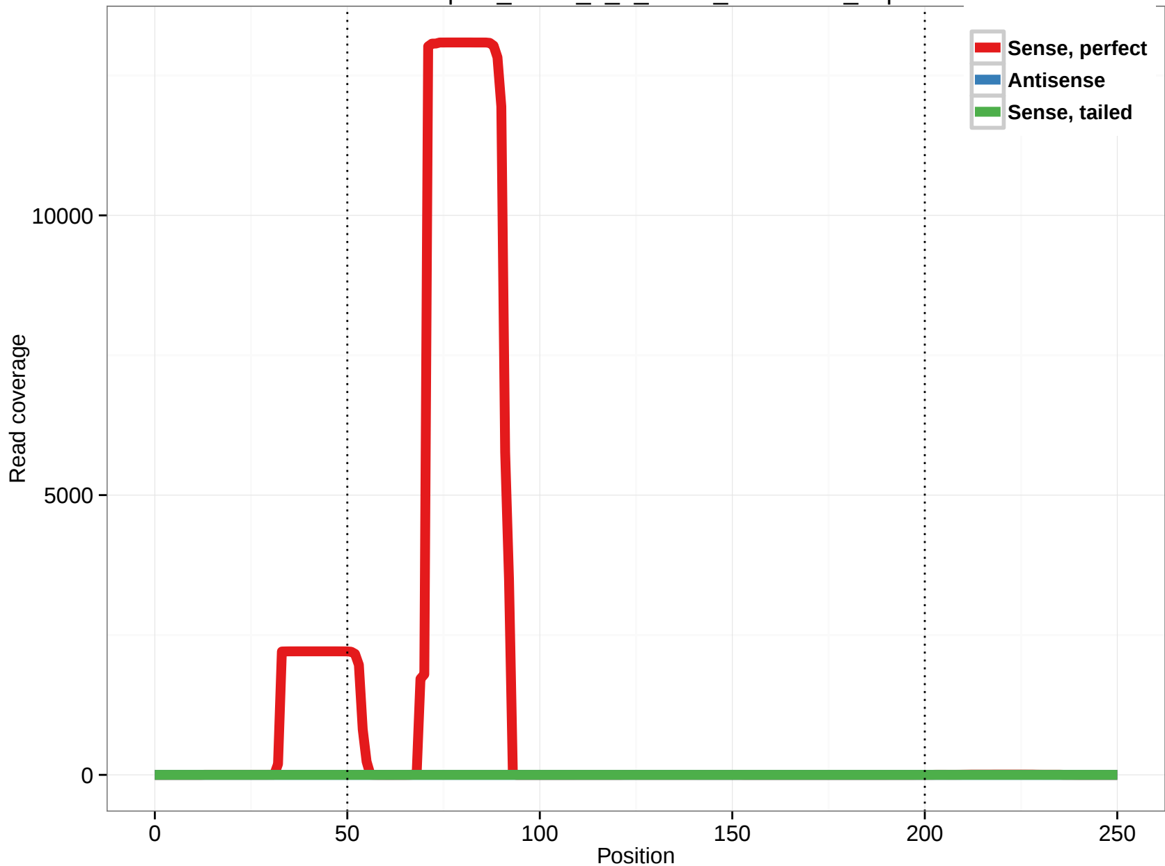
uc001ipk.2_intron_4_0_chr10_17882806_f.3p
