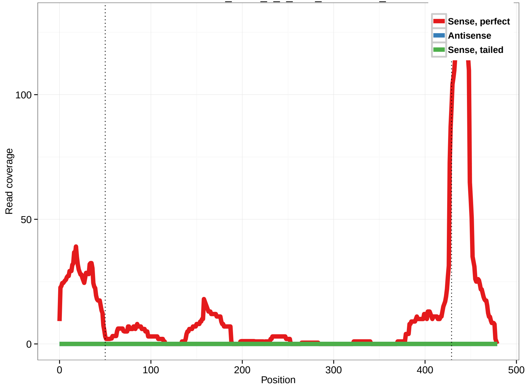
uc001iaw.1_intron_1_0_chr1_245018347_r
