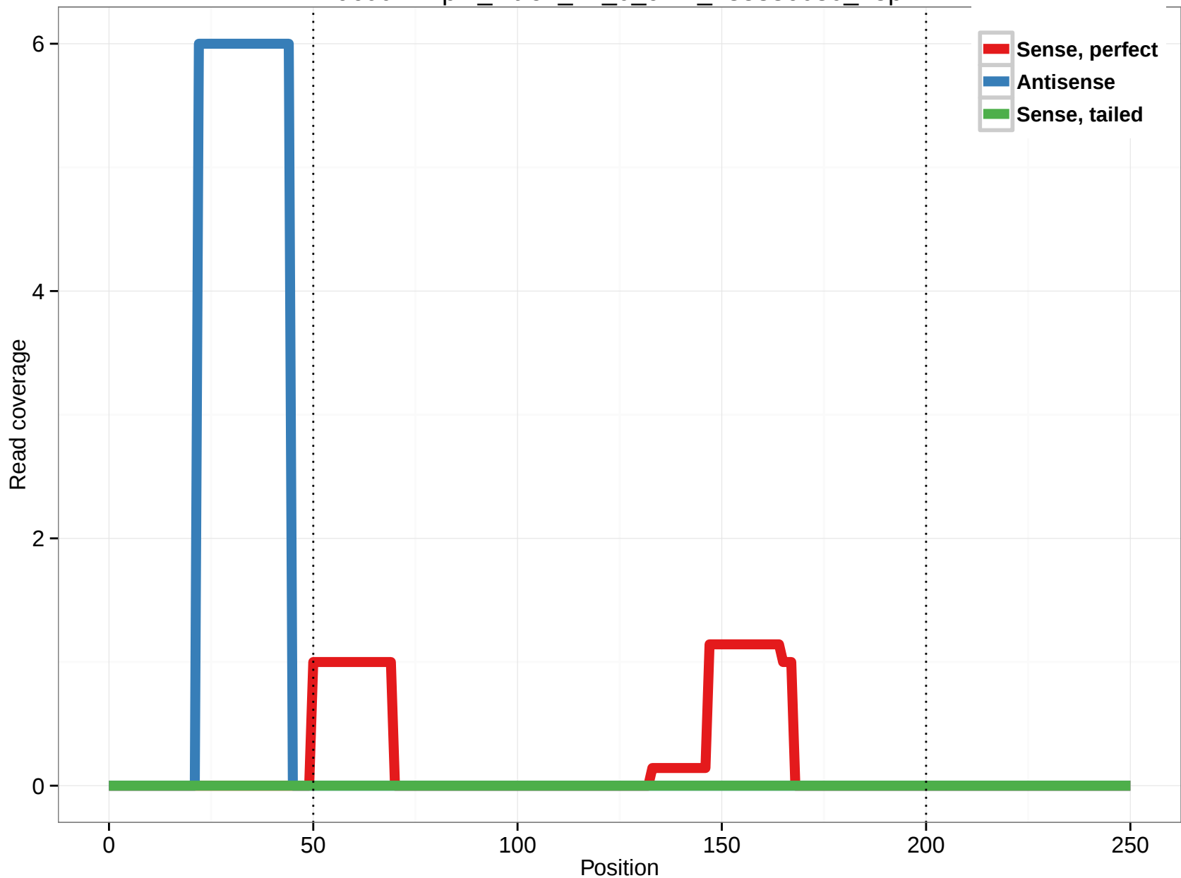
uc001hwp.2_intron_12_0_chr1_235336080_r.5p
