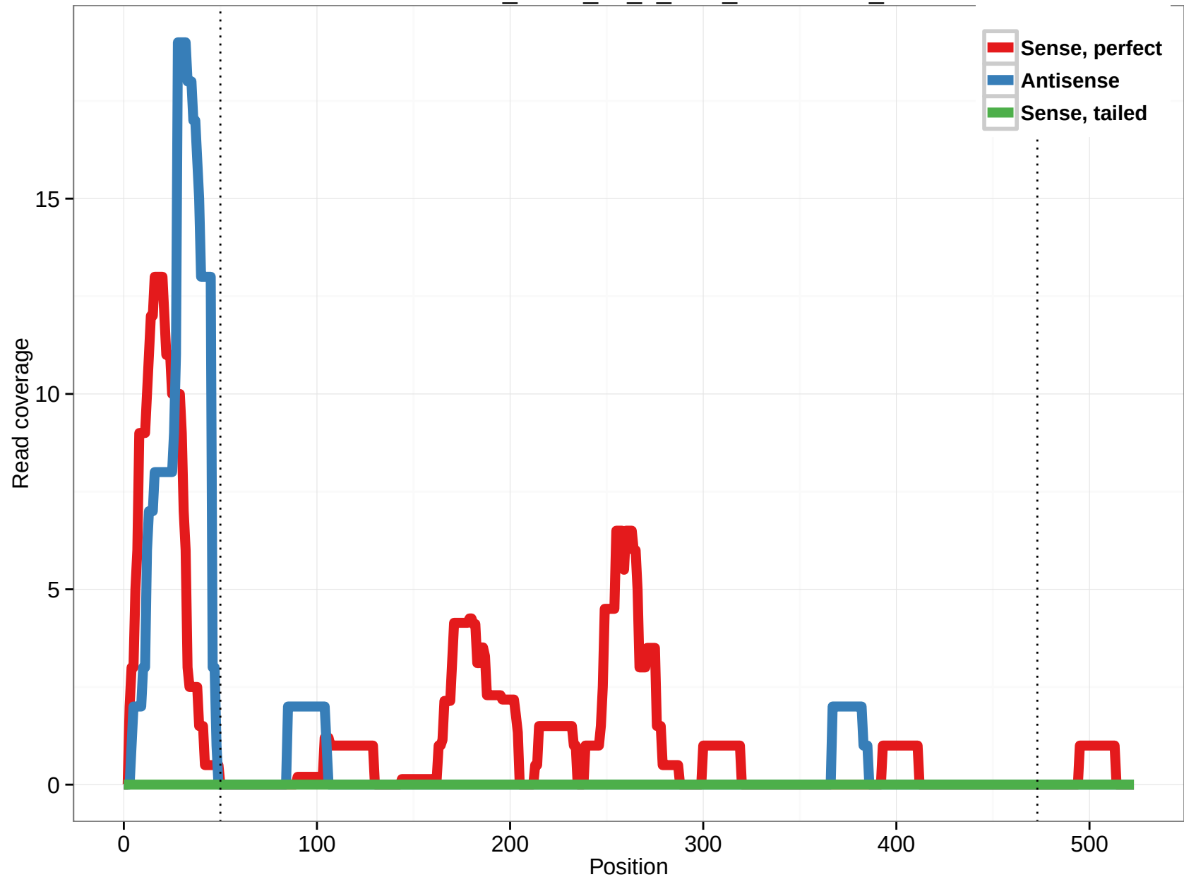
uc001hsn.2_intron_20_0_chr1_228463728_f
