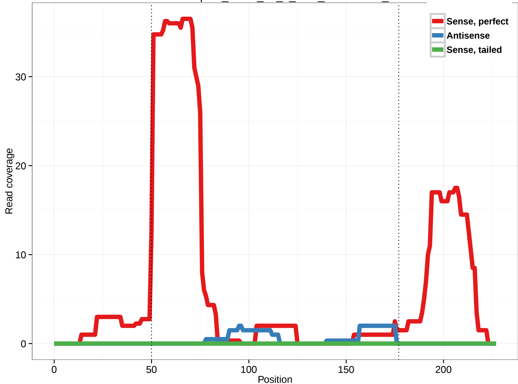
uc001hqm.1_intron_13_0_chr1_227171335_f
