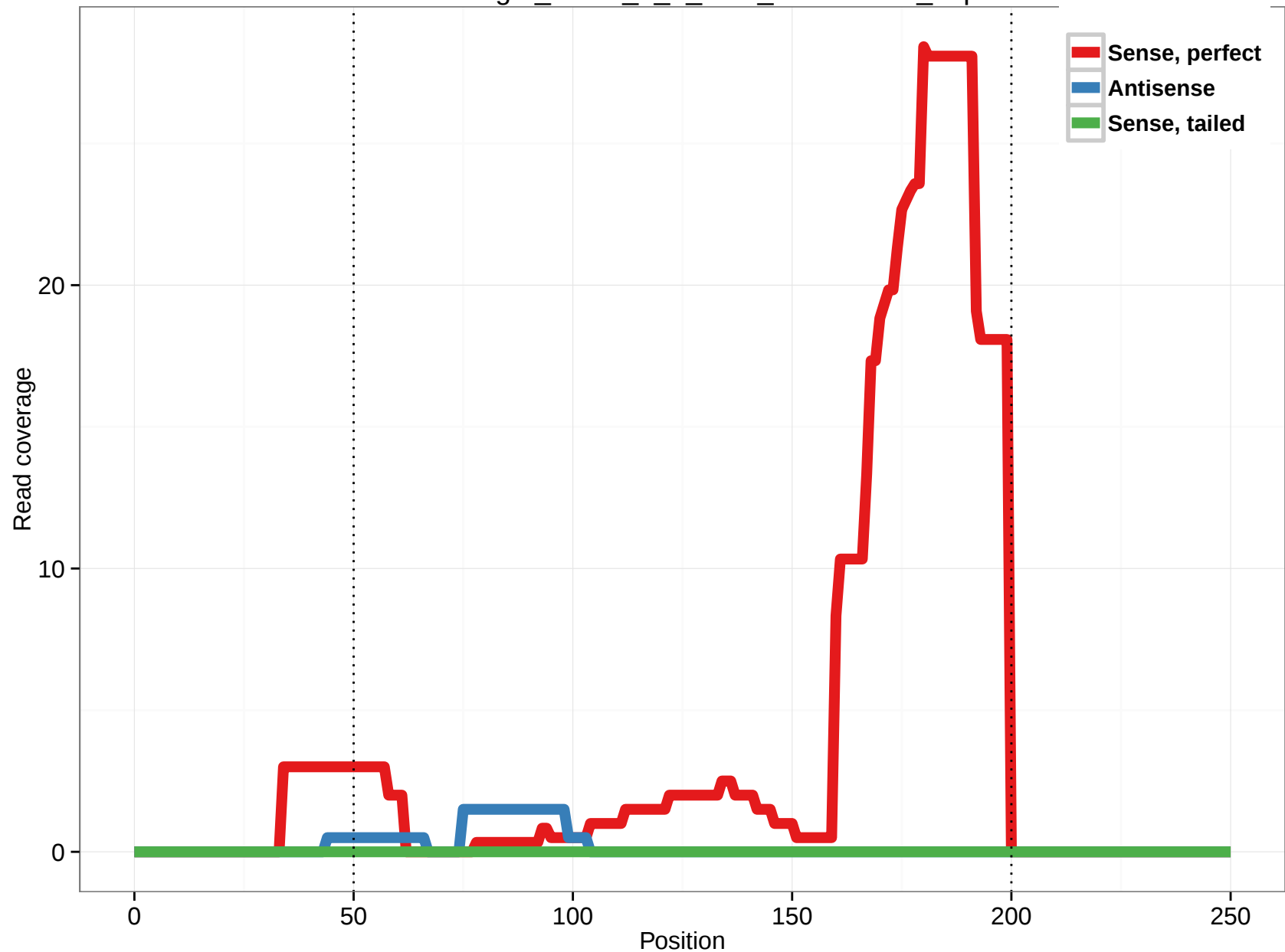
uc001hog.1_intron_1_0_chr1_224195120_f.3p
