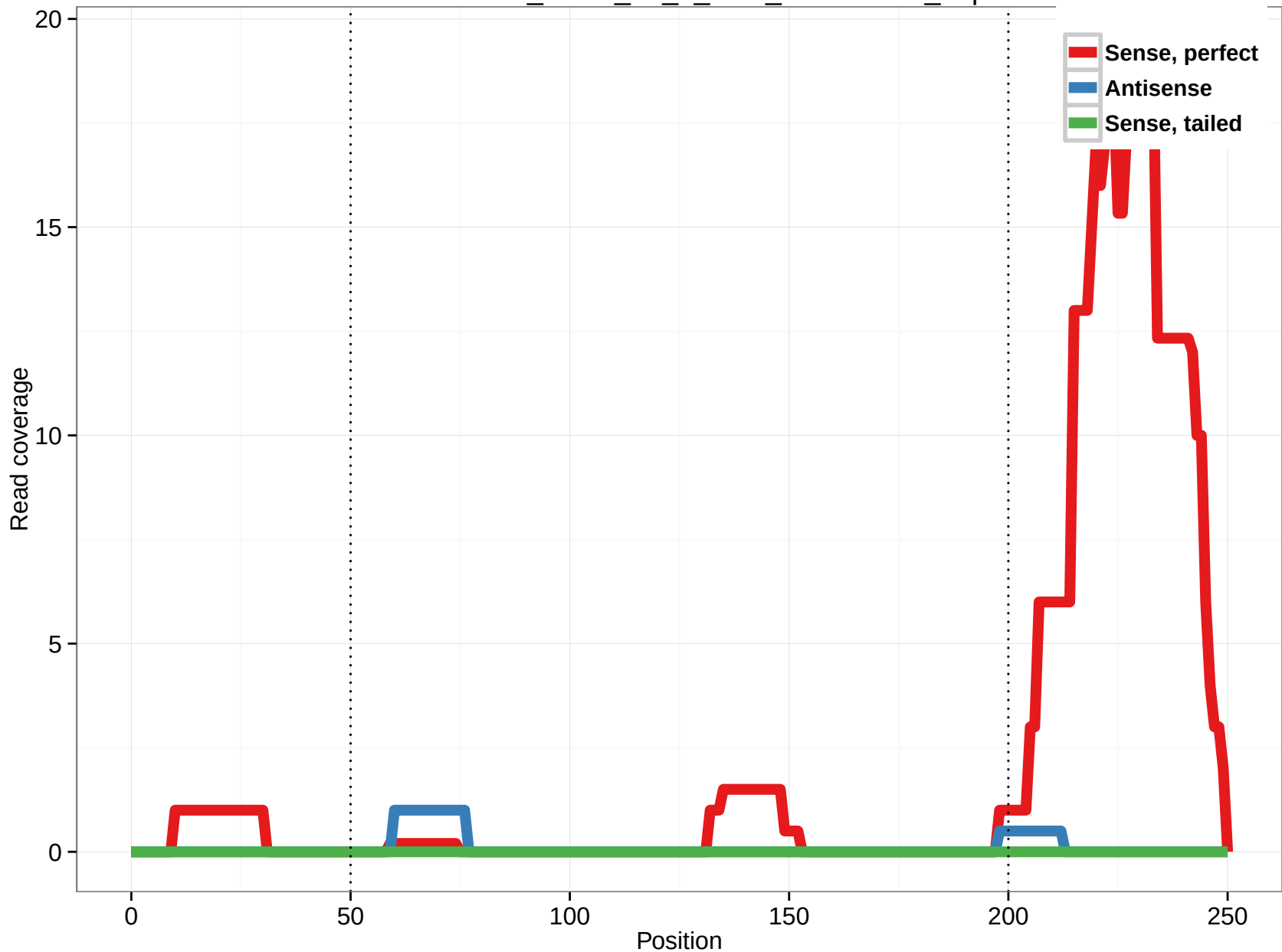
uc001hmc.2_intron_17_0_chr1_220312482_f.3p
