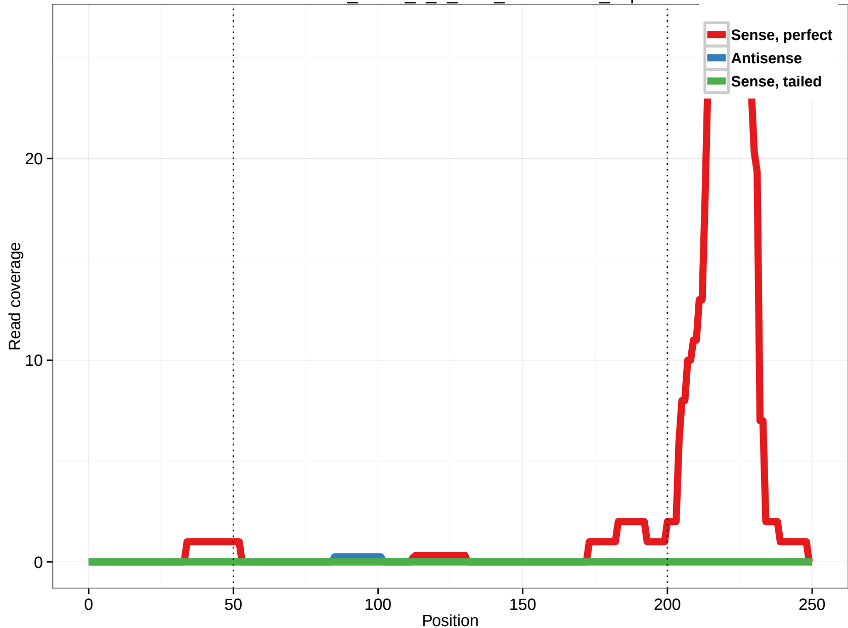
uc001h1r.3_intron_1_0_chr1_219352589_f.3p
