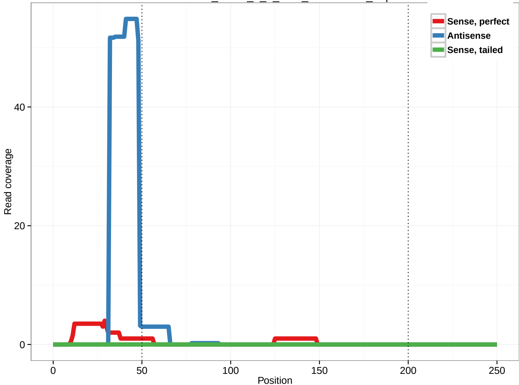
uc001hir.1_intron_0_0_chr1_211836995_r.3p
