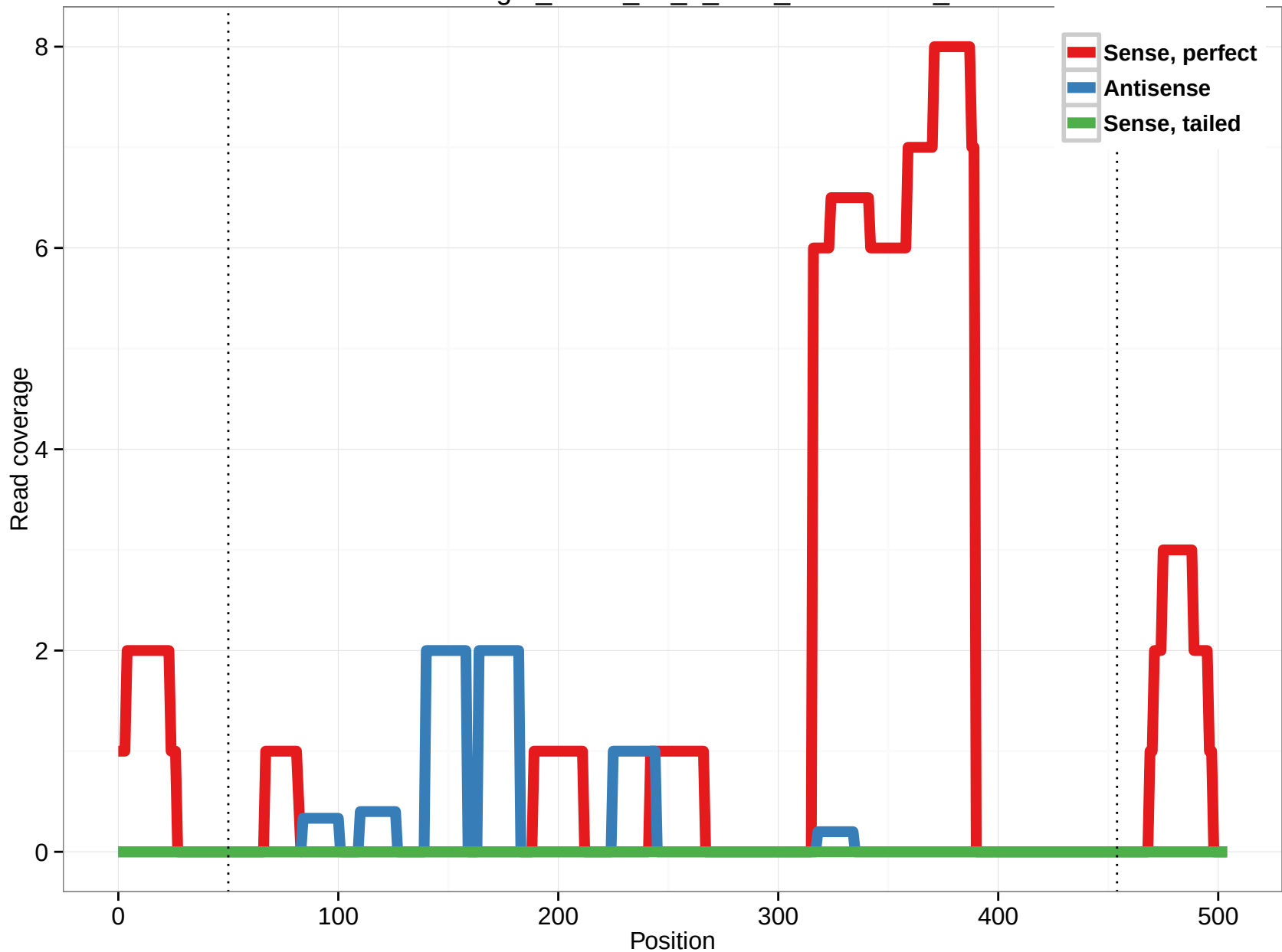
uc001hhg.2_intron_10_0_chr1_209800324_r
